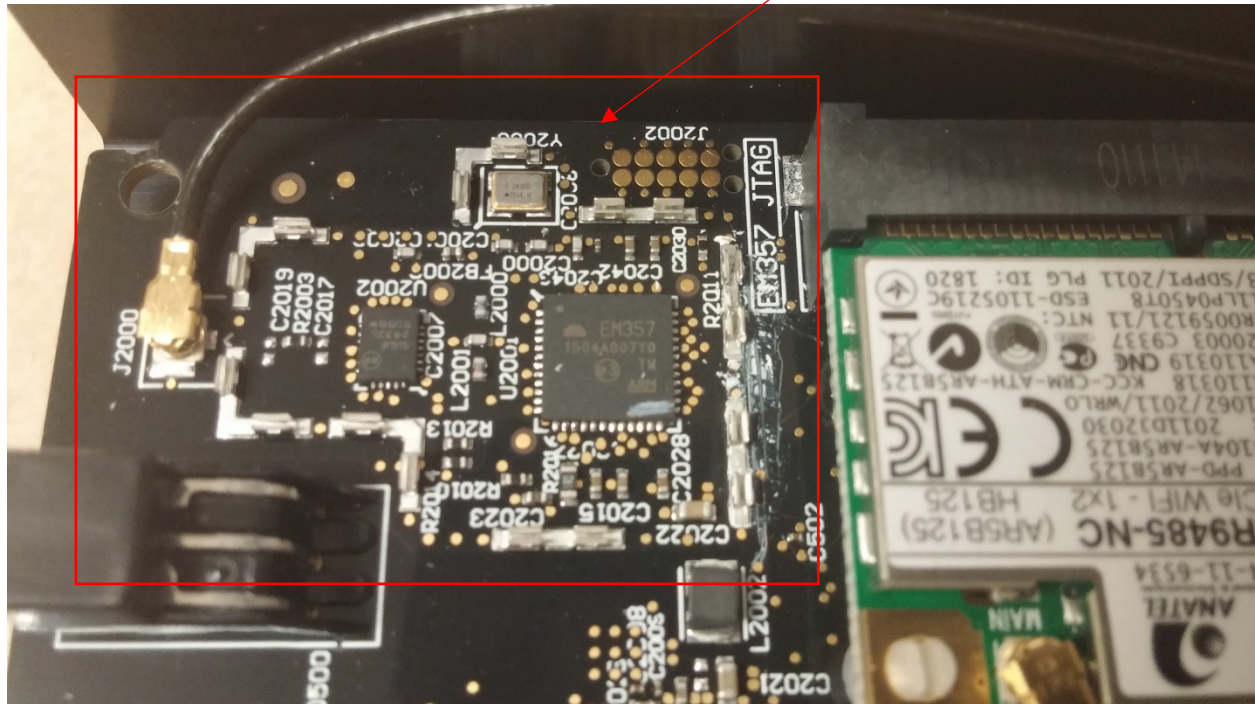
Photograph 12 – View of the 802.15.4 Transceiver Circuitry Under the RF Shield
