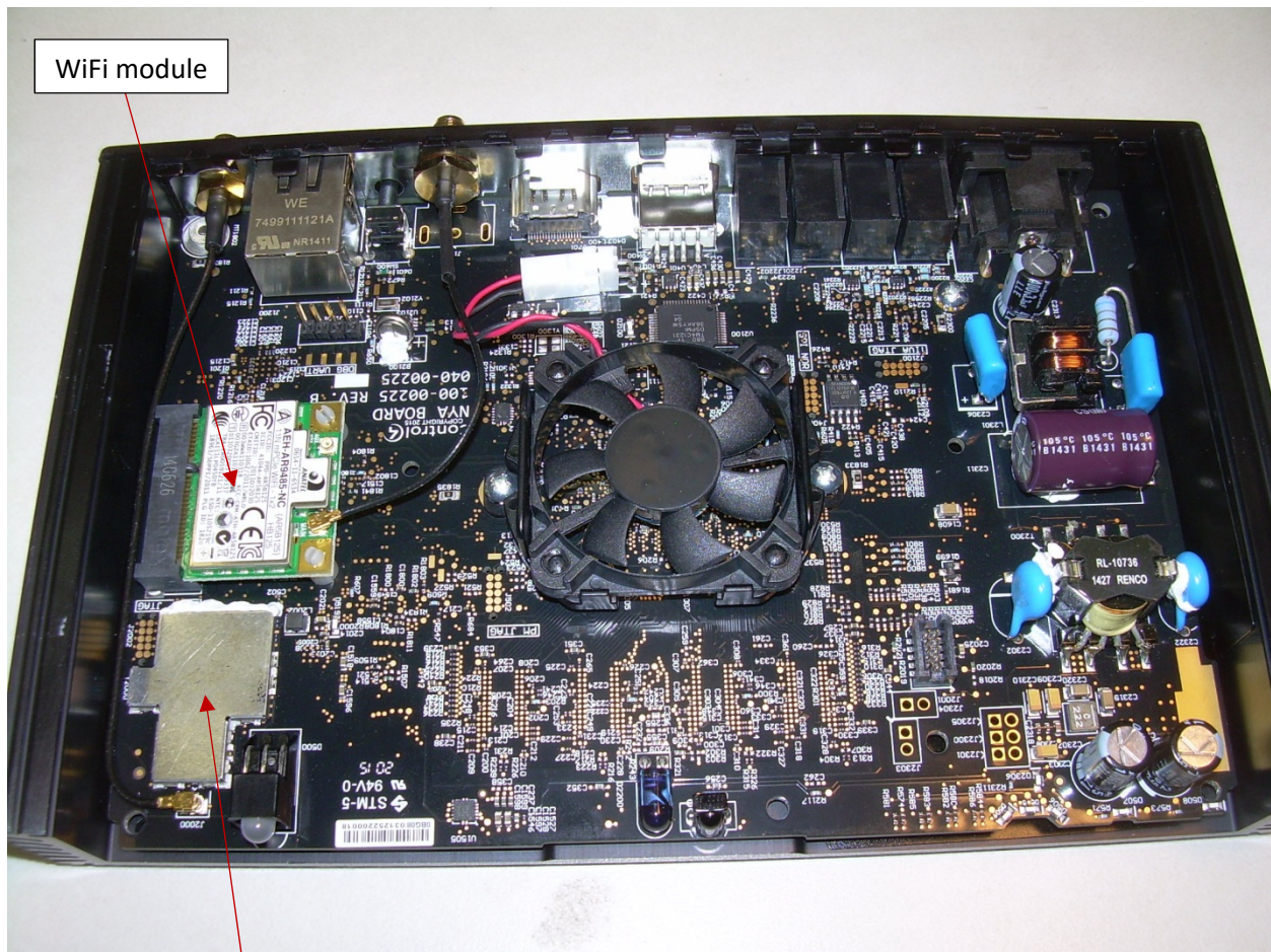
Photograph 10 – View of the EUT with Top Removed Showing Top Side of PCB
