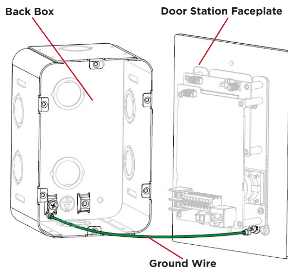
Figure 4. Ground Wires from Door Station to Back Box
