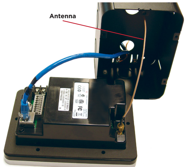
Figure 12. Thread Antenna Through Back Box
