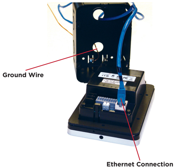
Figure 3. Ethernet with PoE Injector
