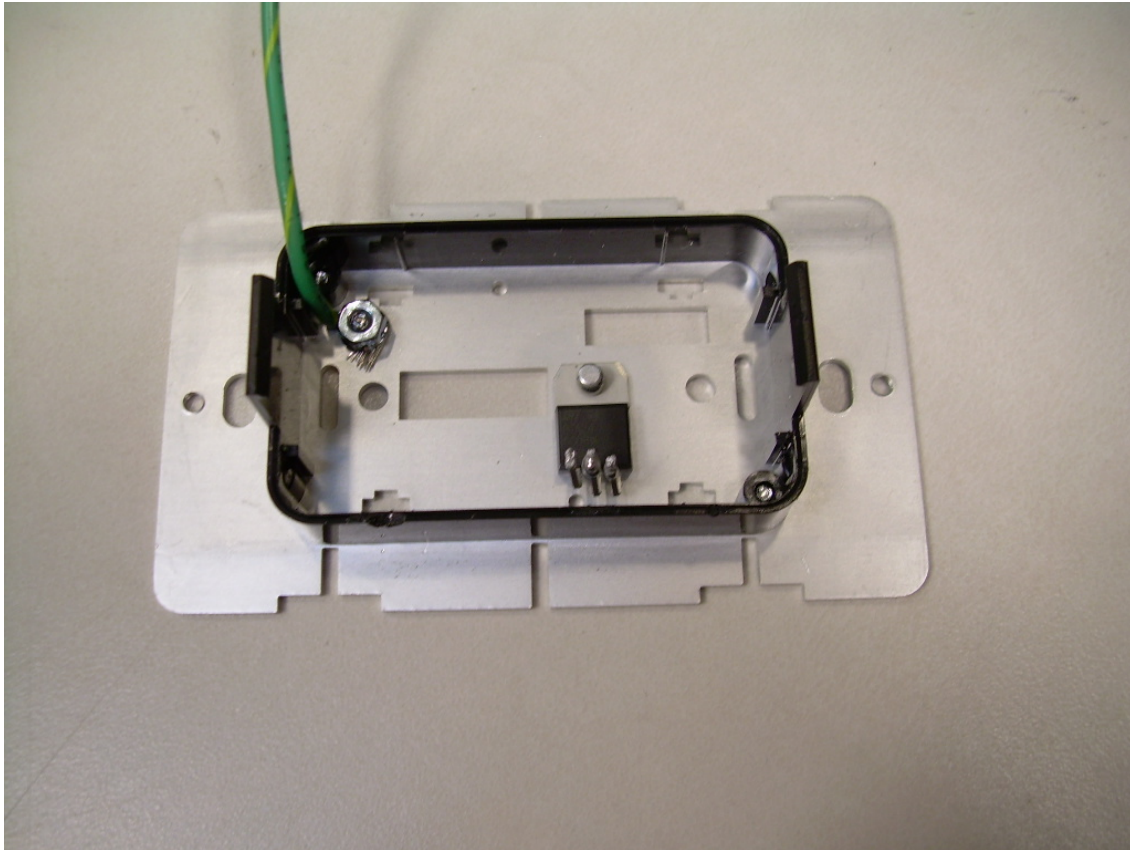
Photograph 12 - View of the Triac Mounting
