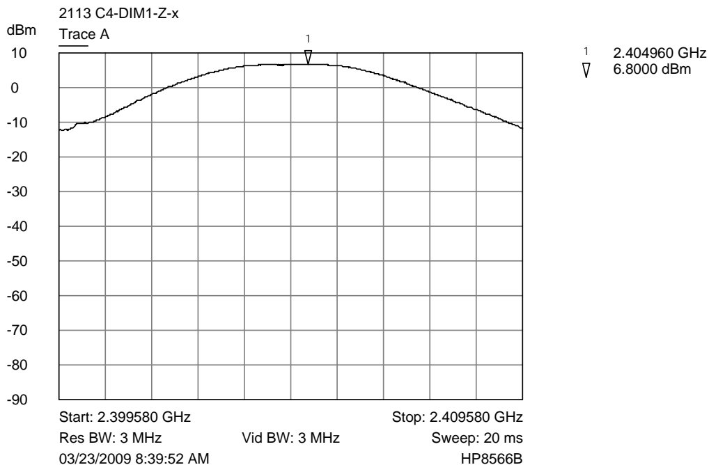
Trace A Lower channel output power
