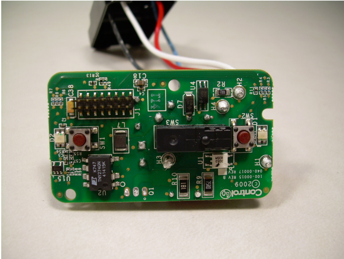
Photograph 11 - View of the Front of the Main Dimmer PCB
