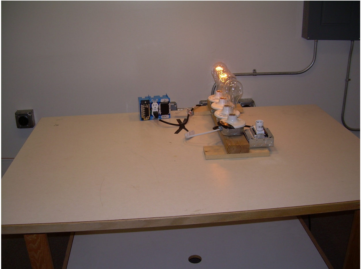
Front View Conducted Disturbance Worst Case Configuration
