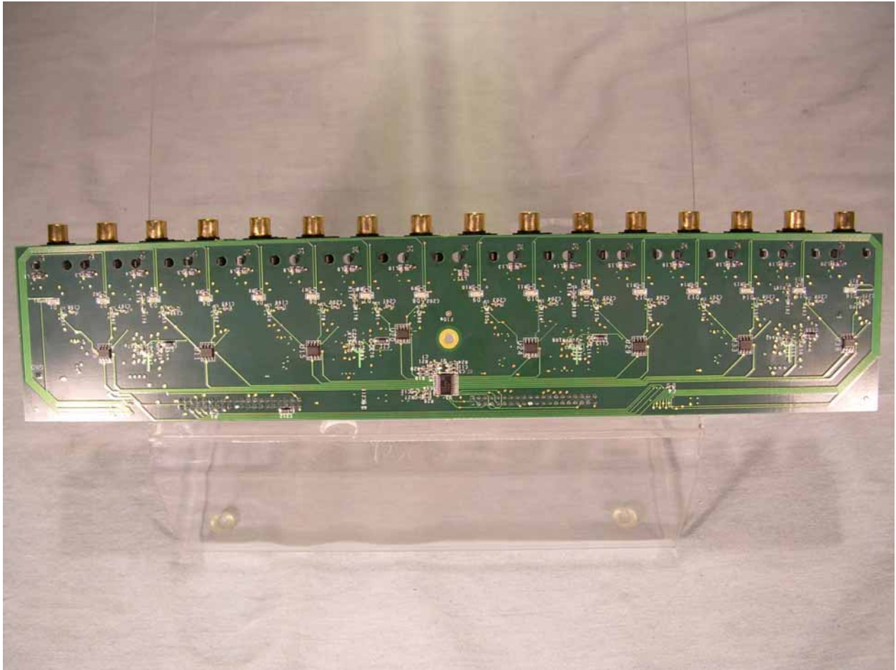
Bottom Side of the Rear Panel Interface PCB
