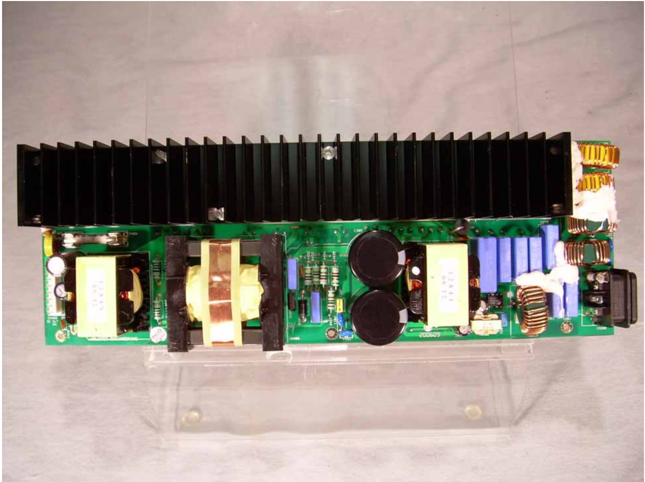
Top Side of the Power Supply
