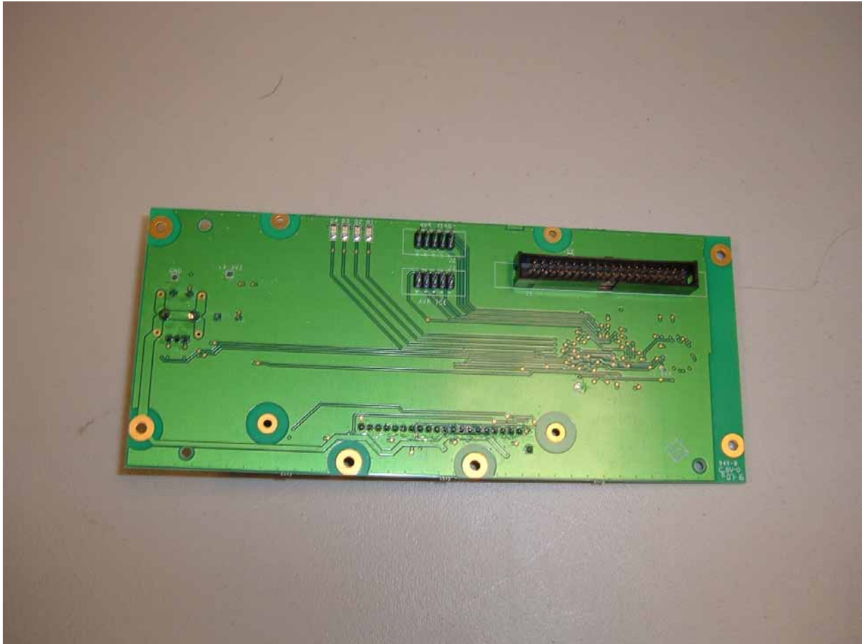
Back Side of the Front Panel PCB
