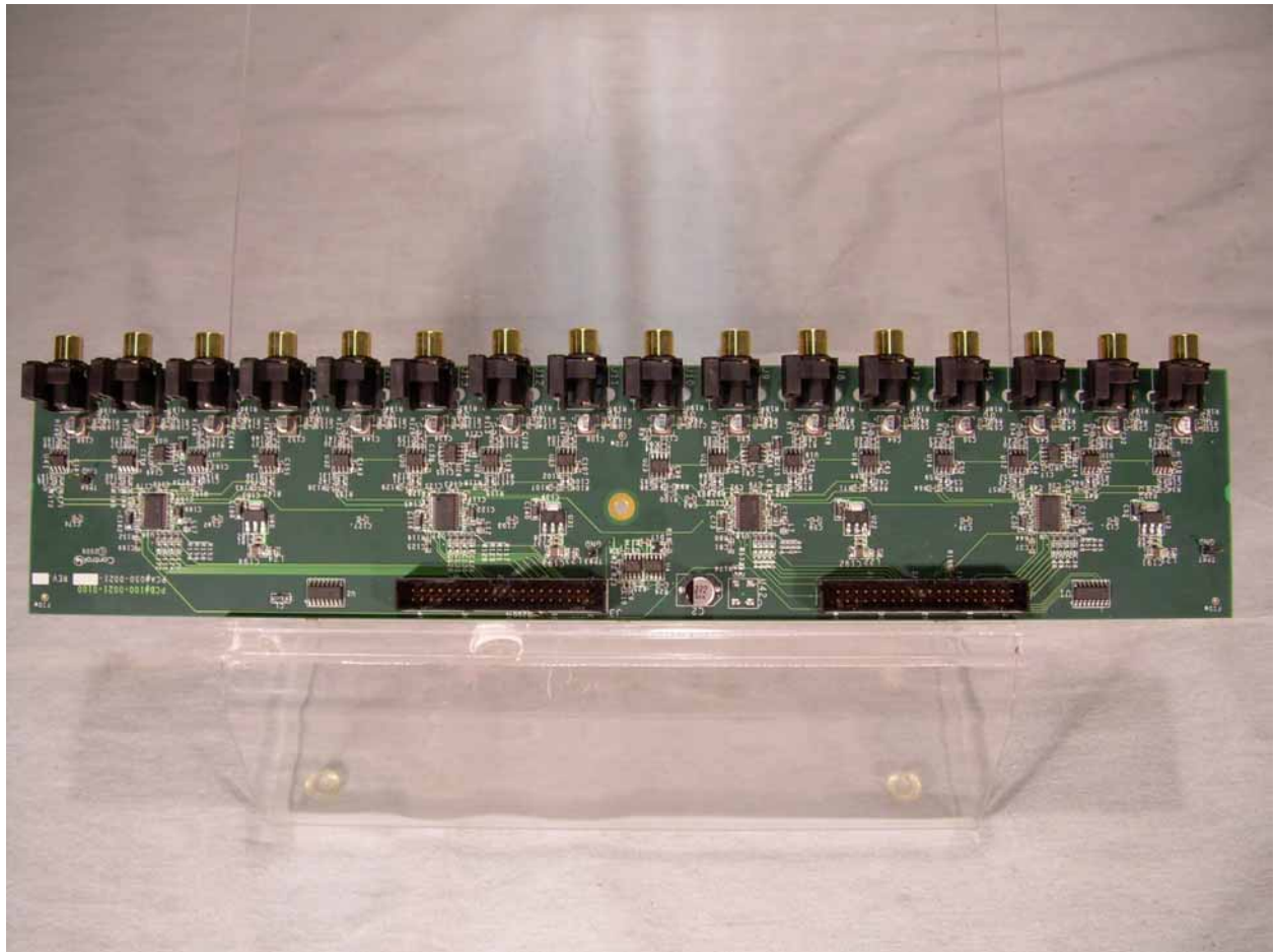
Top Side of the Rear Panel Interface PCB
