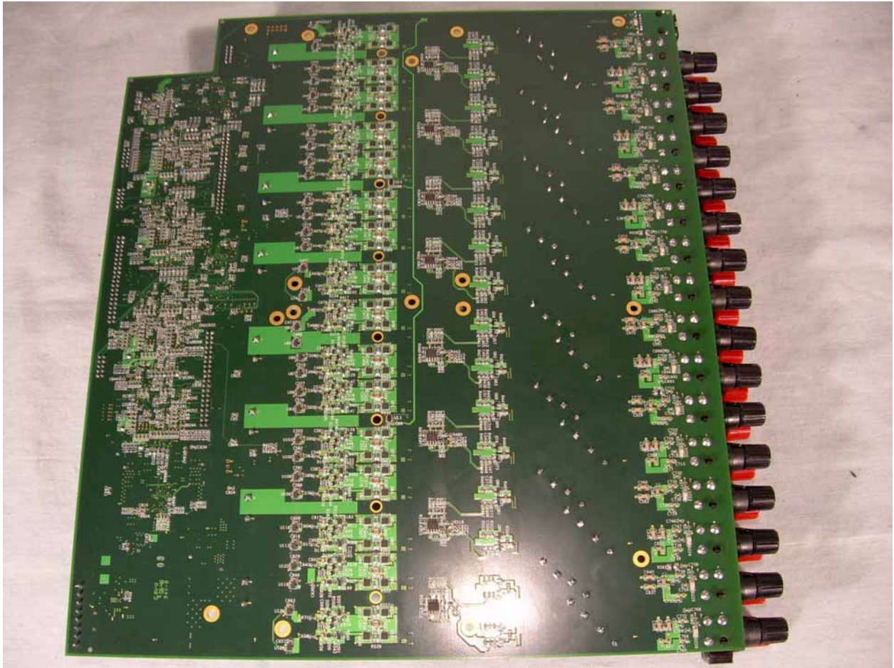
Bottom Side of the Main PCB
