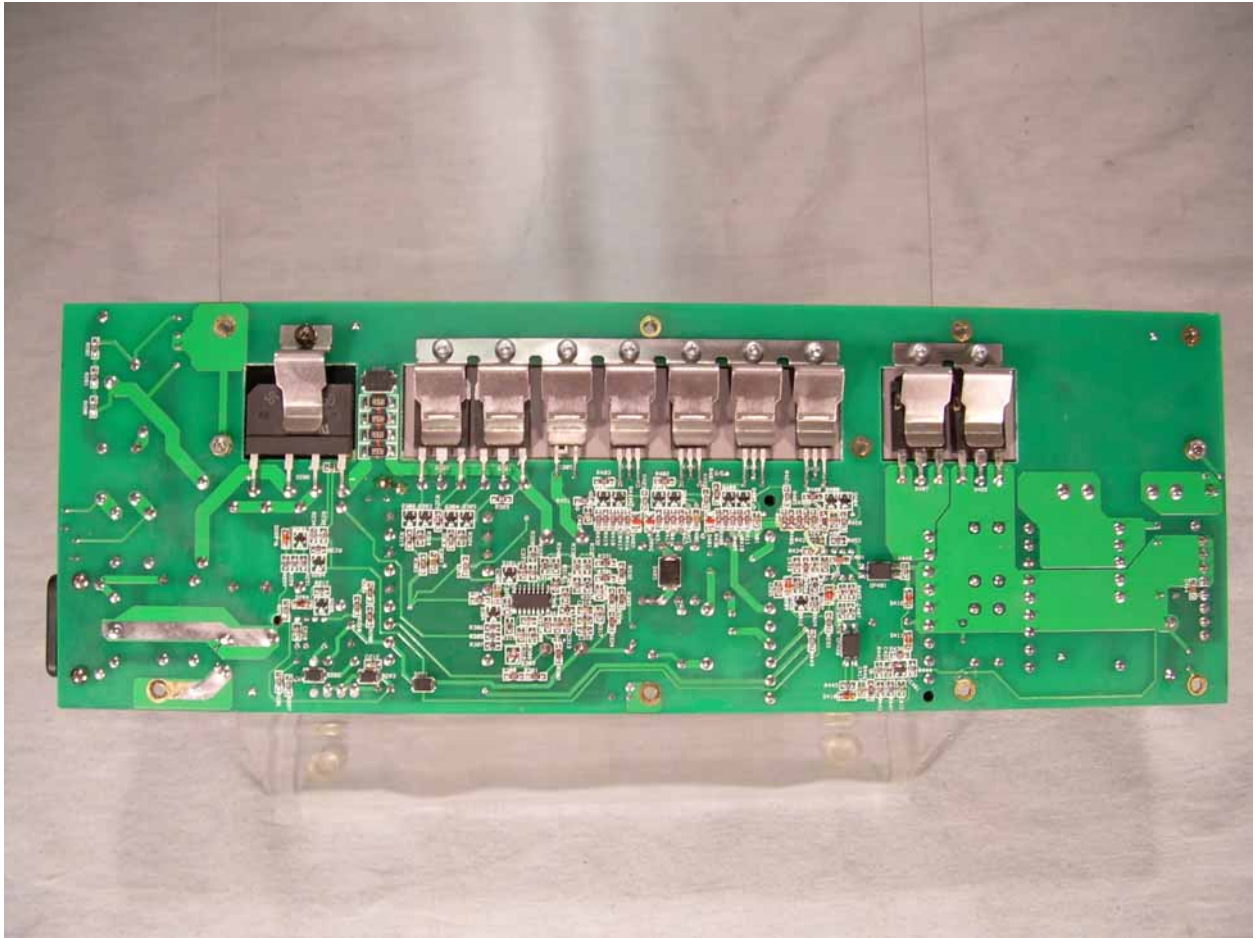
Bottom Side of the Power Supply
