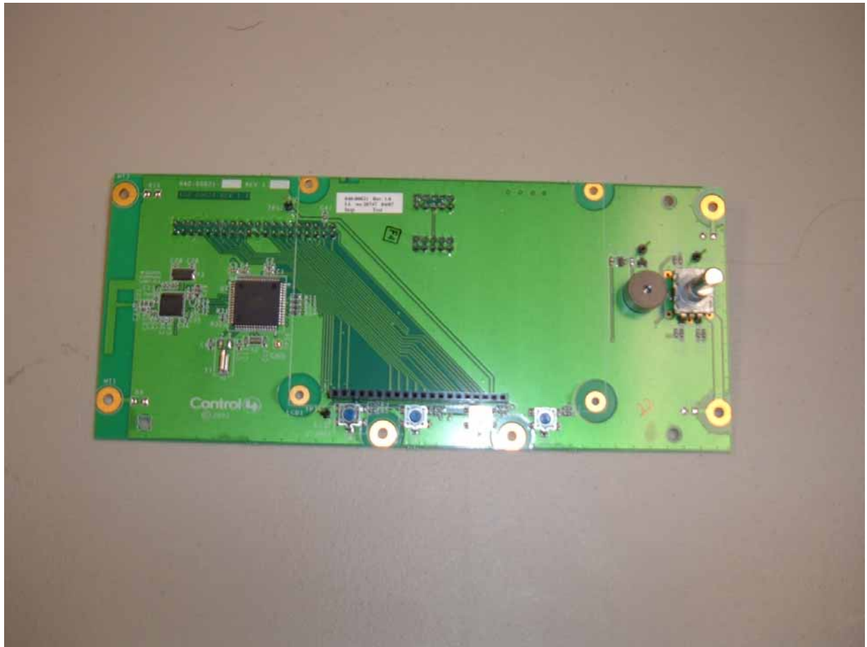
Front Side of the Front Panel PCB
