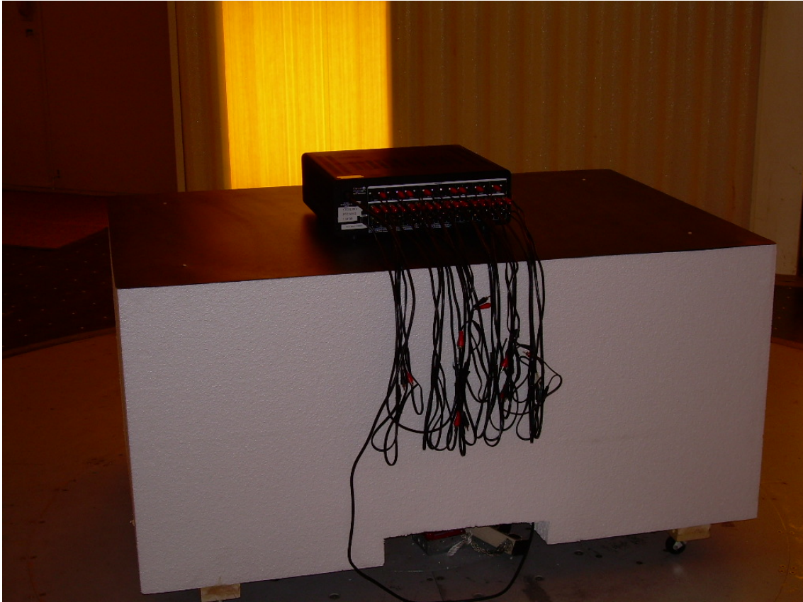
Back View Radiated Spurious Emission Test Configuration
