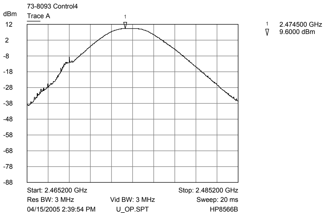
Trace A Upper Channel Output Power Plot
