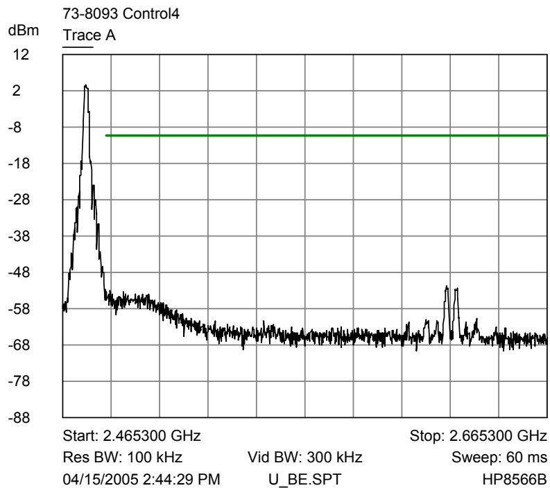
Trace A Upper Channel Upper Band Edge Plot
