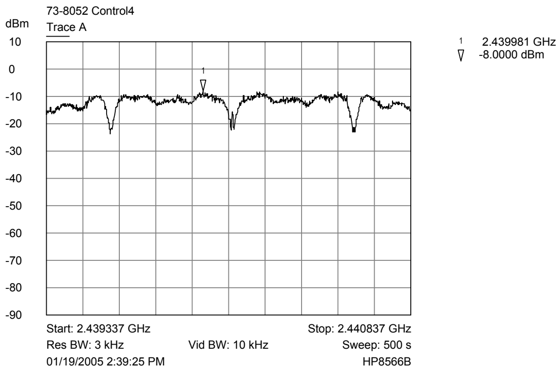
Trace A Middle channel 3kHz power spectral density
