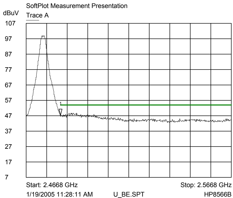
Trace A upper band edge radiated
