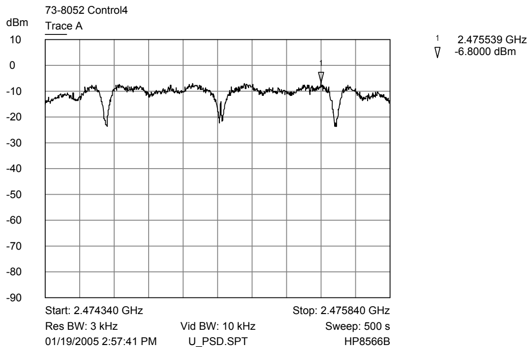
Trace A Upper channel 3kHz power spectral density
