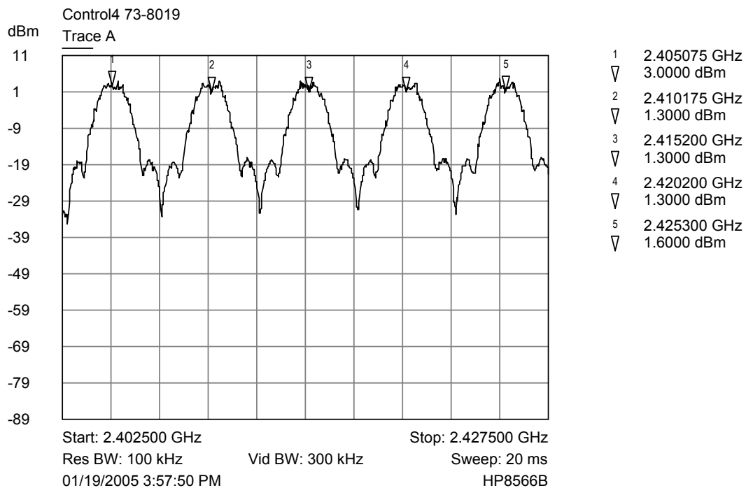
Trace A Lower 5 channels
