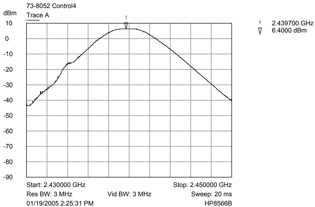
Trace A Middle channel output power
