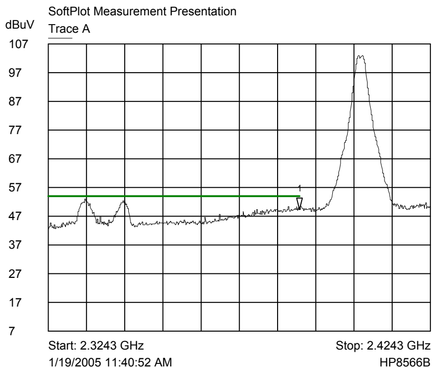
Trace A lower band edge radiated
