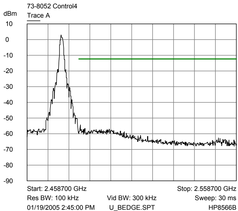
Trace A Upper channel band edge
