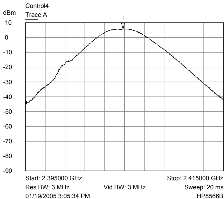
Trace A Lower channel output power
