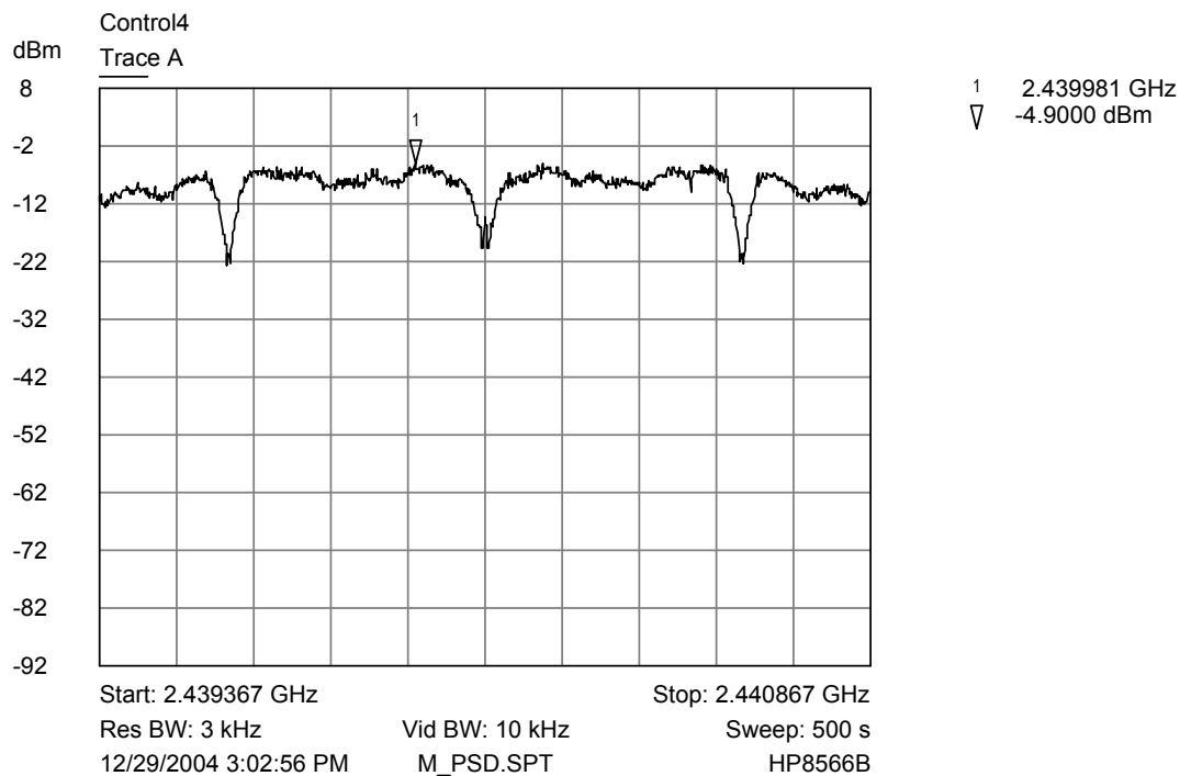
Roadrunner mid channel 3kHz power spectral density
