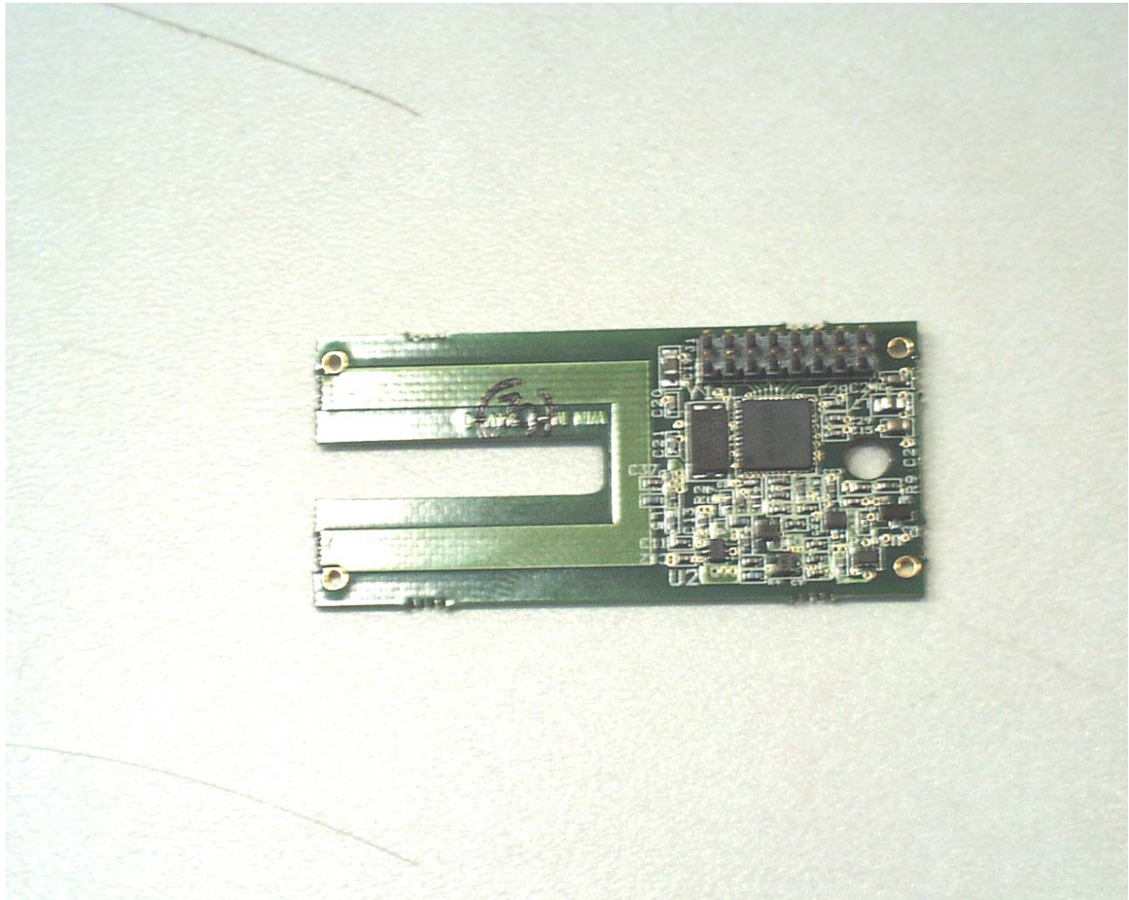
Photograph 8 - Component Side of the Radio Card
