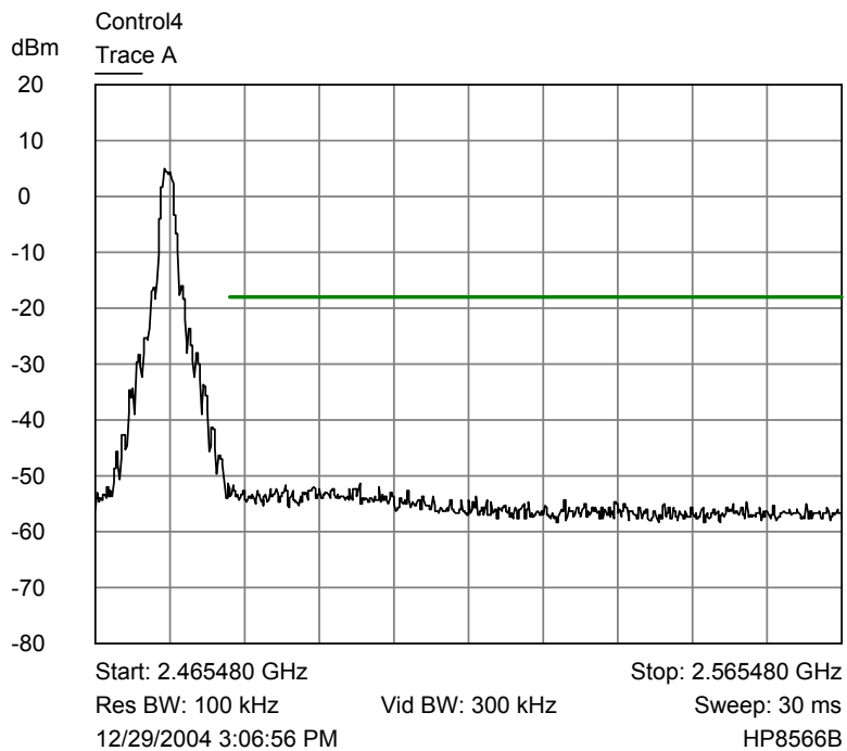
Roadrunner upper channel band edge
