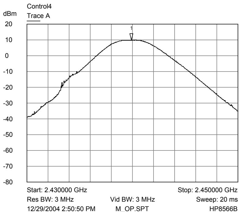
Roadrunner mid channel output power
