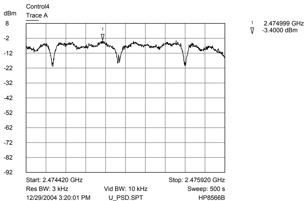
Roadrunner upper channel 3kHz power spectral density
