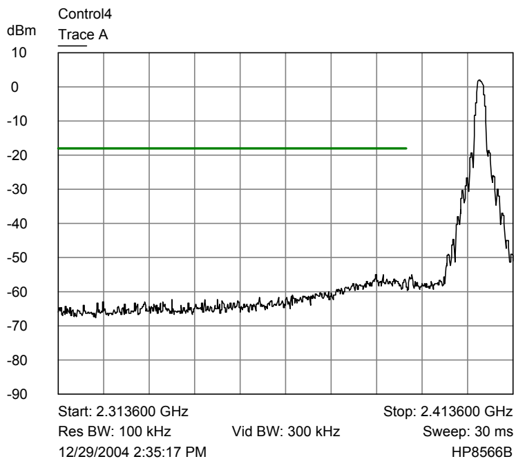
Roadrunner lower band edge plot
