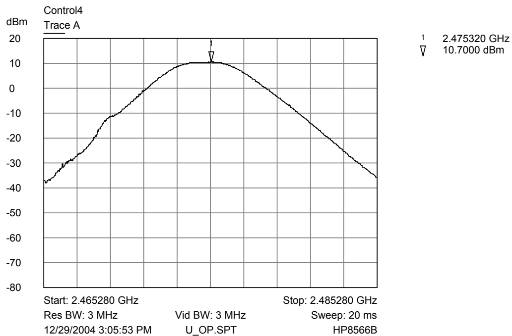
Roadrunner upper channel output power
