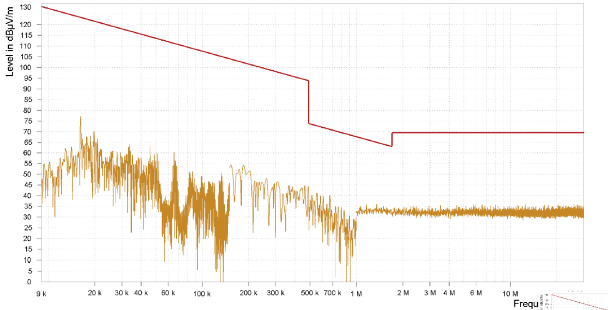
Radiated Spurious Emission 9 kHz – 30 MHz (Antenna Position 180°) : BLE 2M (CH 0)
