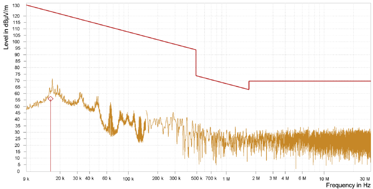
Radiated Spurious Emission 9 kHz – 30 MHz (Antenna Position 180°) : BLE 2M (CH 0)
