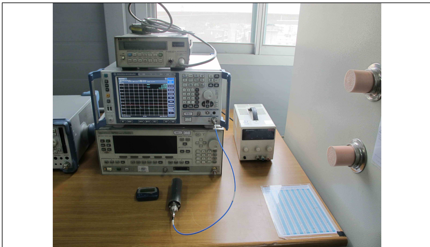
RF Test
