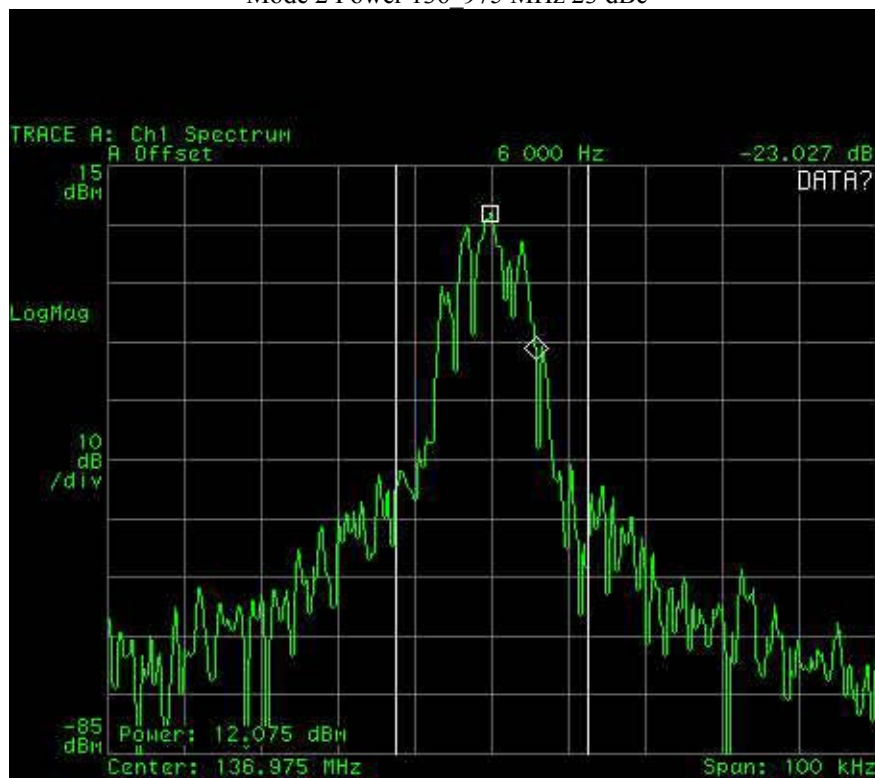
Mode 2 Power 136.975 MHz 23 dBc
