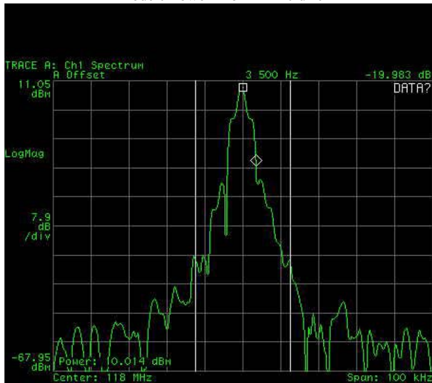
Mode 0 Power 118 MHz 20 dBc
