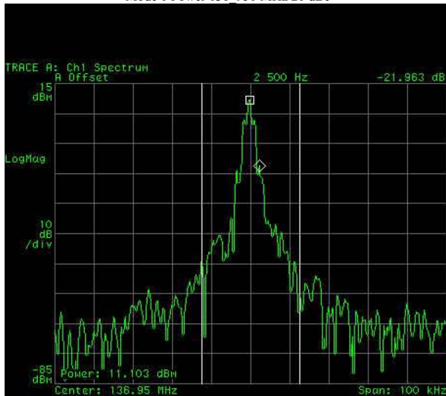
Mode 0 Power 136.950 MHz 20 dBc
