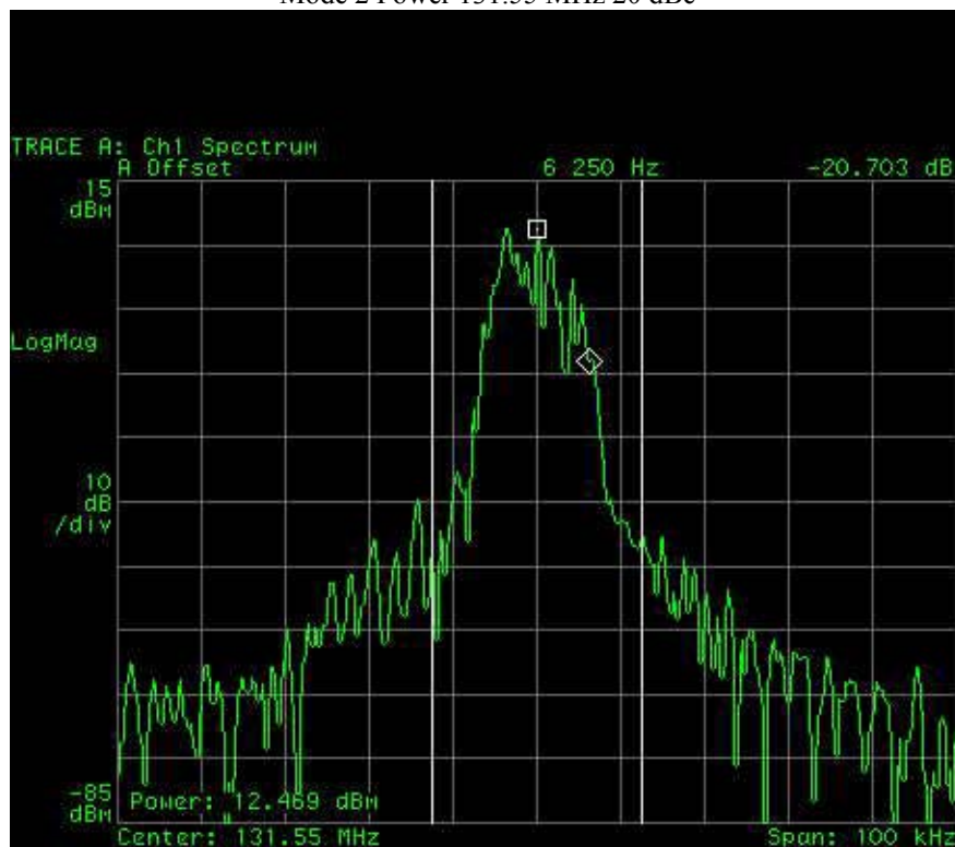
Mode 2 Power 131.55 MHz 20 dBc
