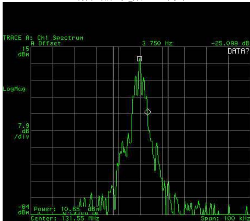
Mode o Power 131.550 MHz 25 dBc
