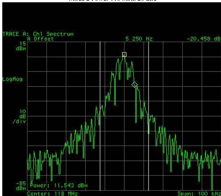
Mode 2 Power 118 MHz 20 dBc
