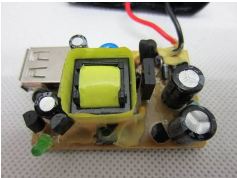
INTERNAL PHOTO OF POWER SUPPLY – 2
