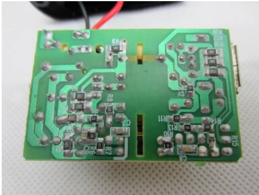
INTERNAL PHOTO OF POWER SUPPLY – 3
