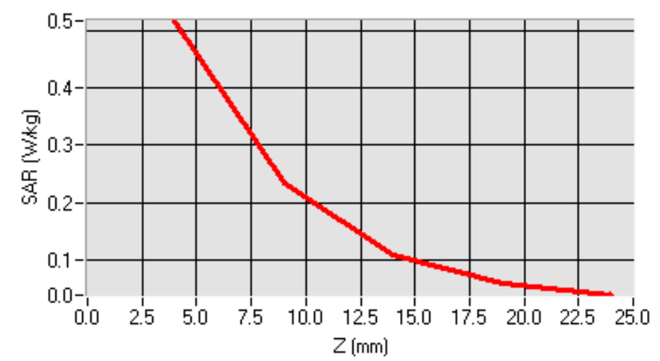
SAR, Z Axis Scan (X = 7, Y = 2)
