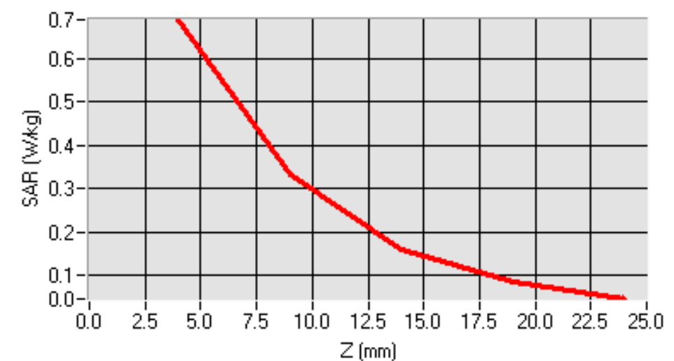
SAR, Z Axis Scan (X = -14, Y = 9)
