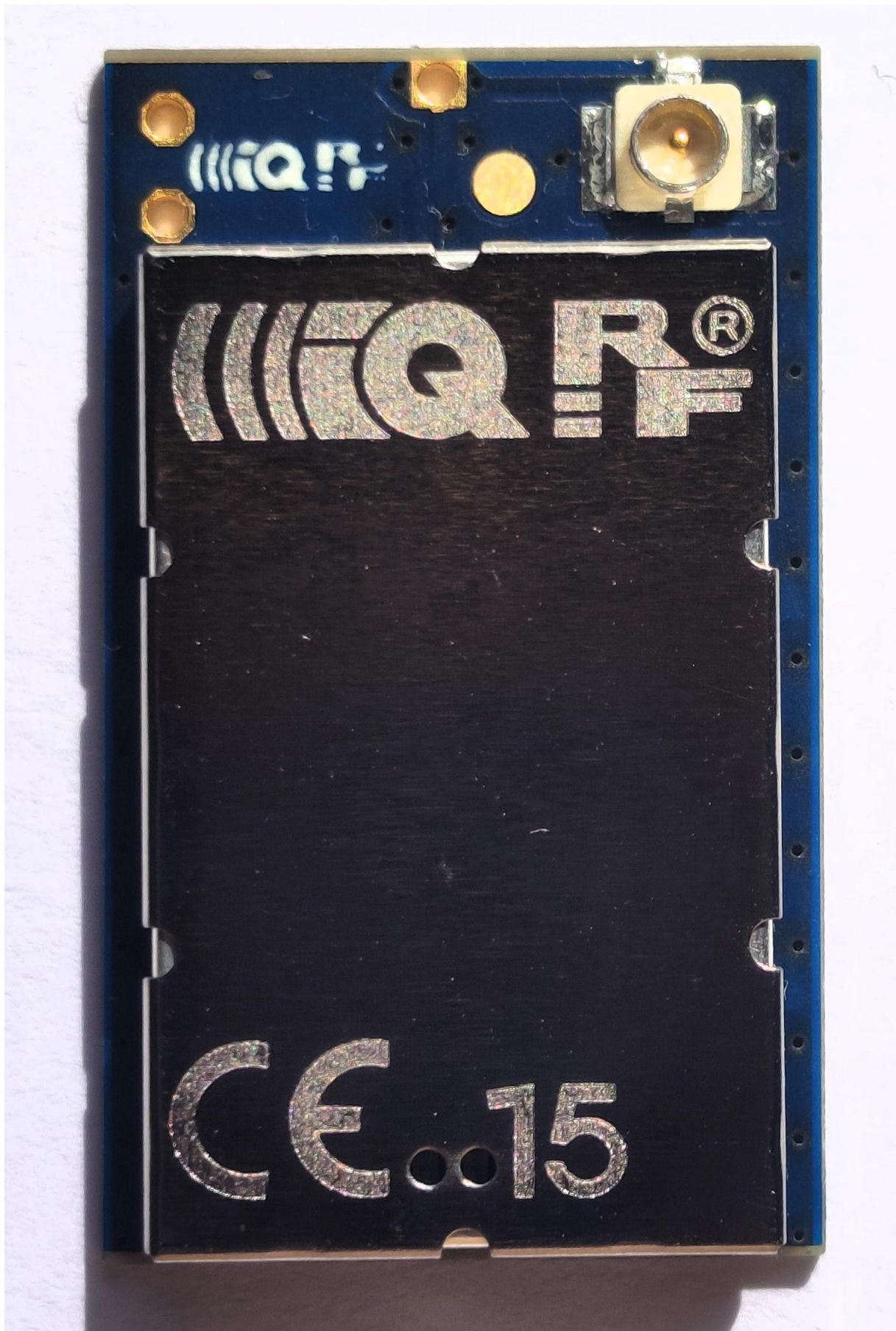
Figure 4: TR-82G, TOP with shield
