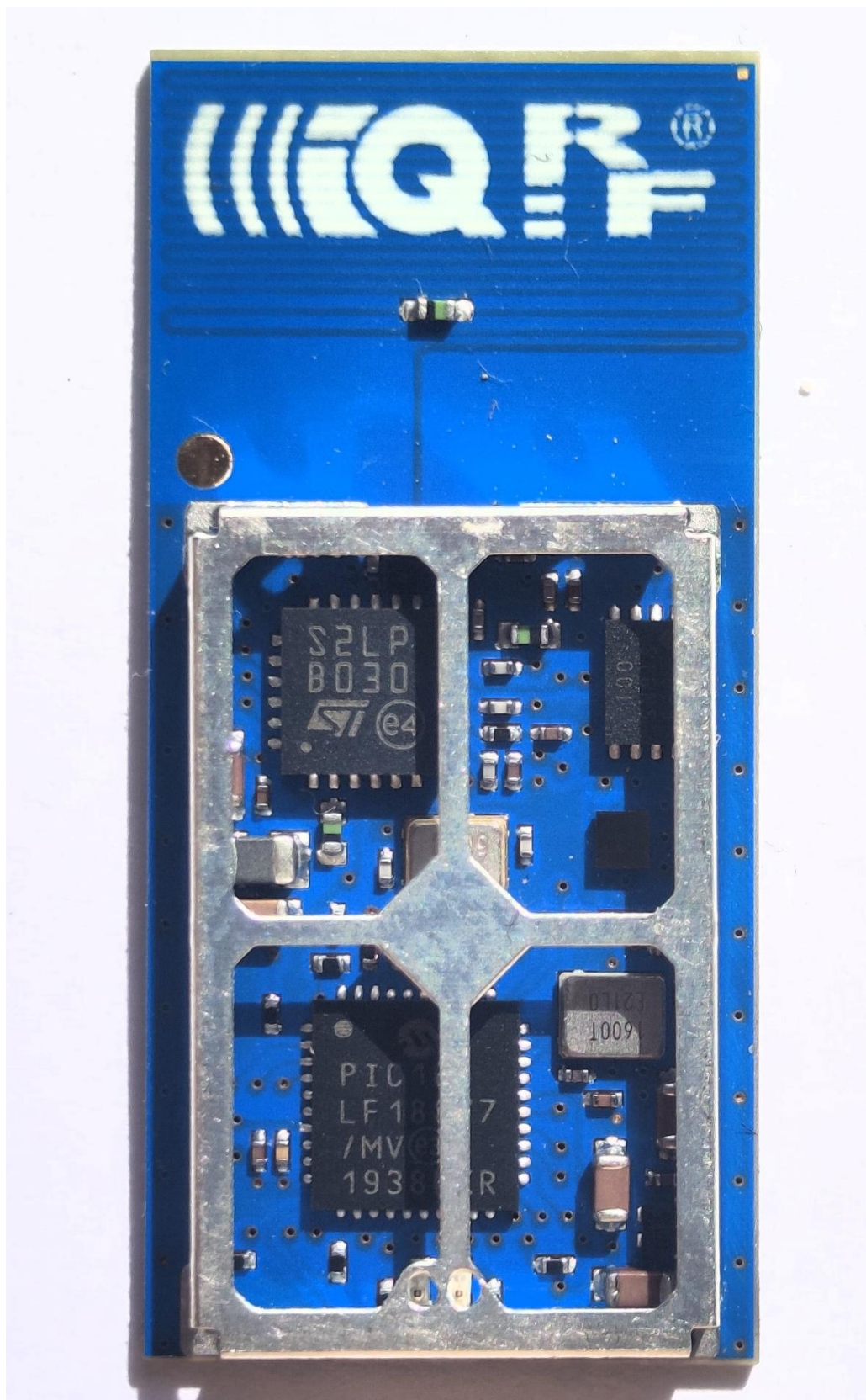
Figure 2: TR-82GA, TOP
