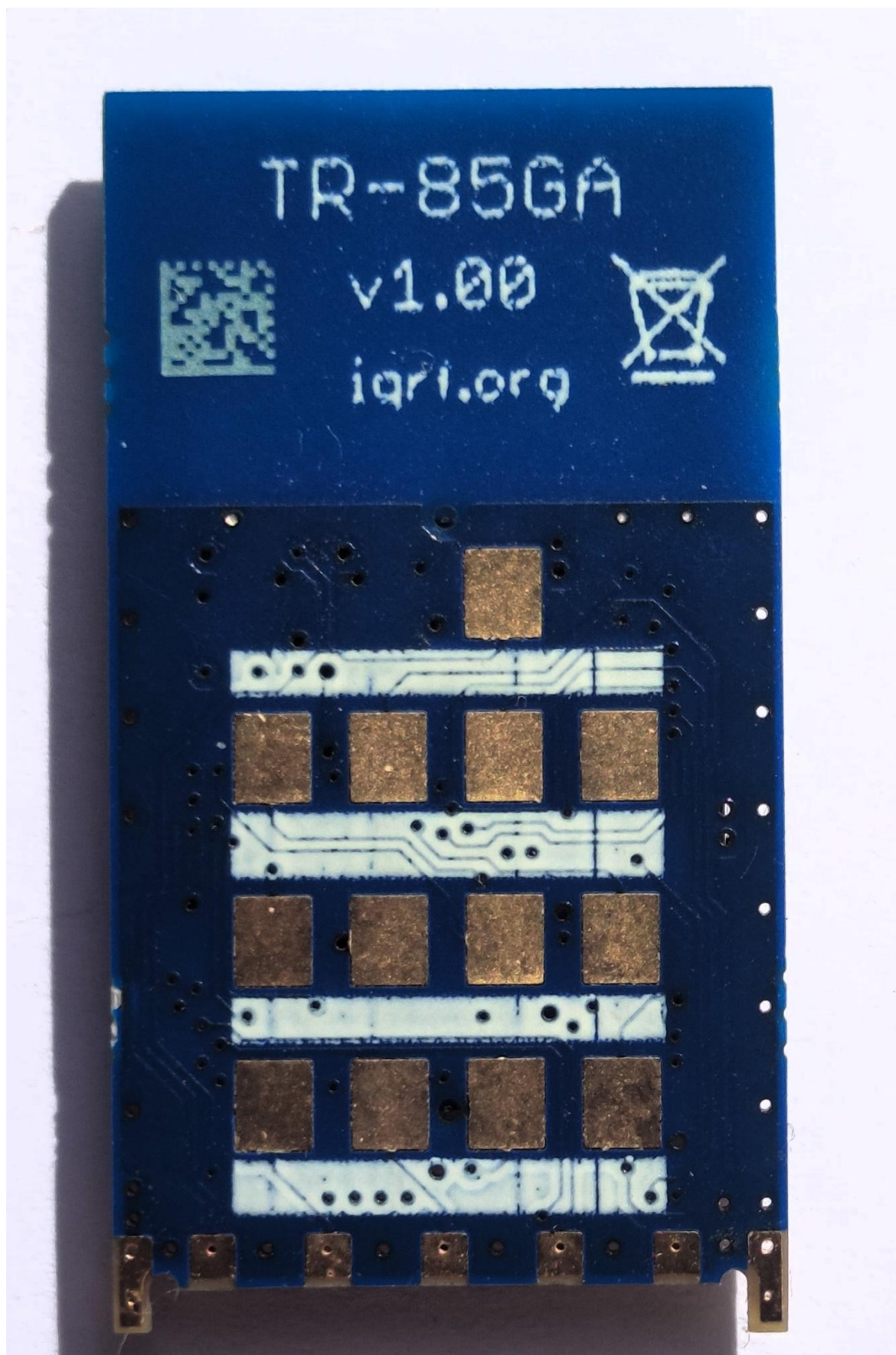
Figure 15: TR-85GA, BOT
