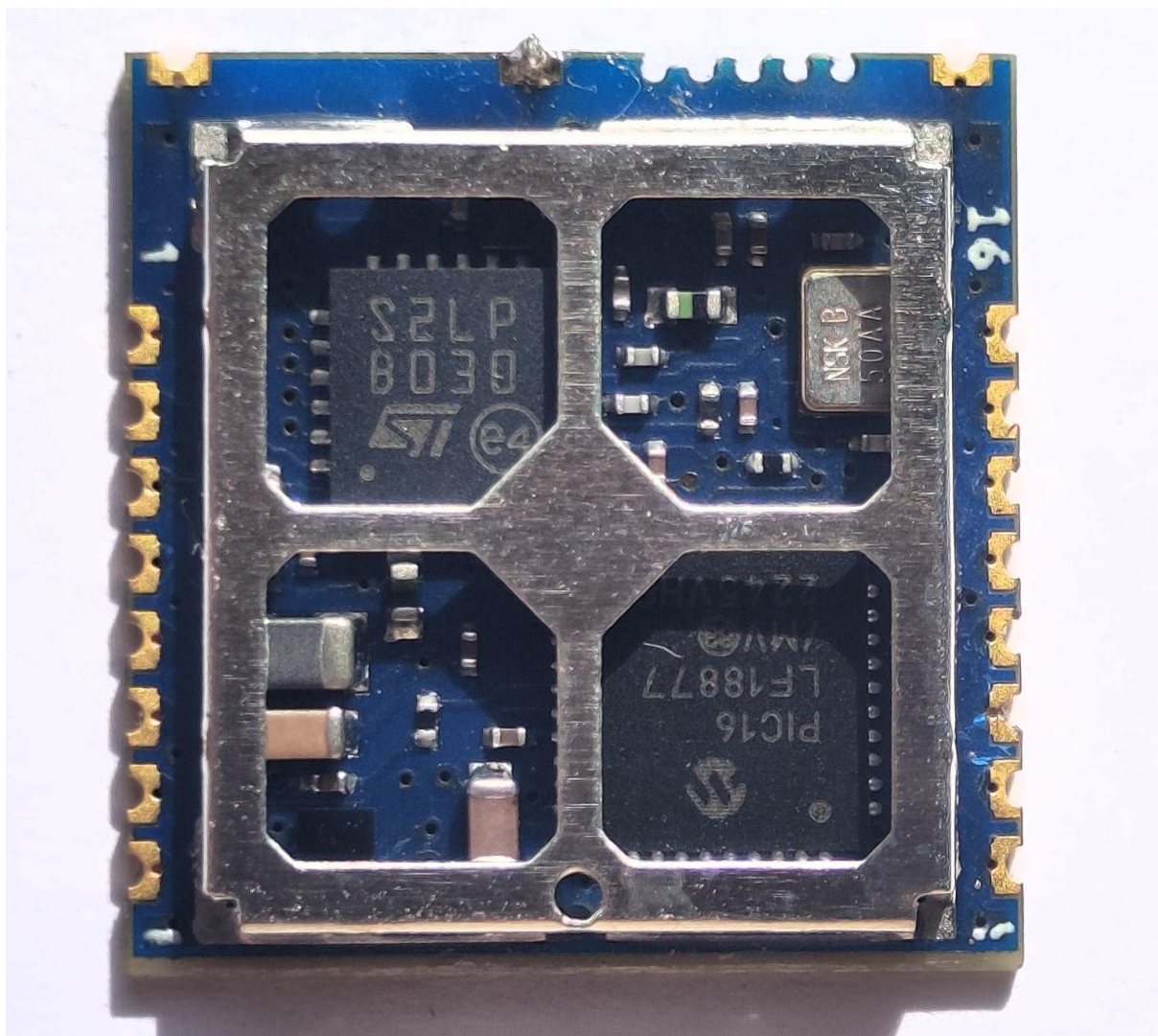
Figure 11: TR-86G, TOP
