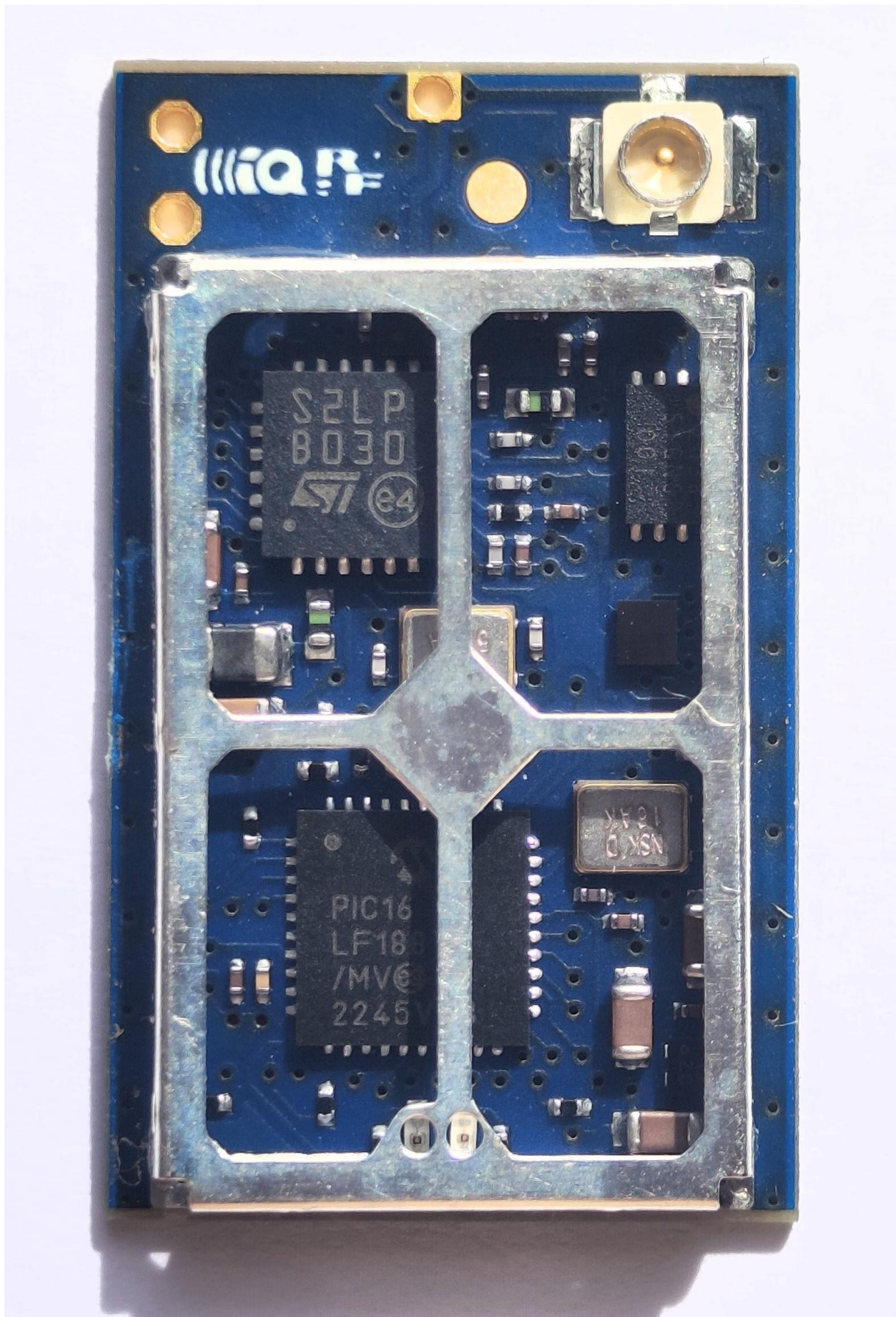
Figure 5: TR-82G, TOP
