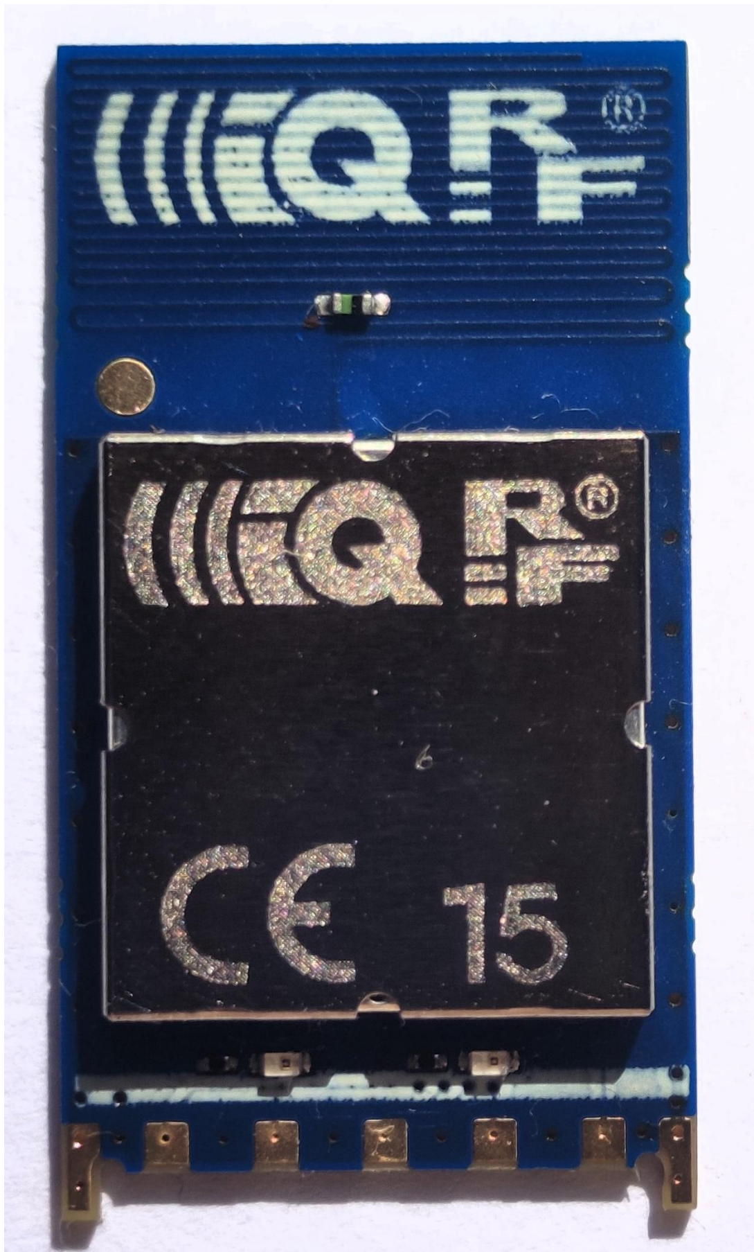
Figure 13: TR-85GA, TOP with shield
