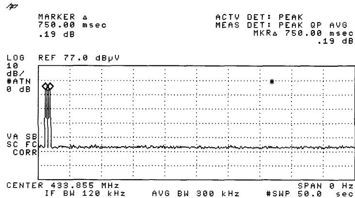
Periodic operation [FCC 47CFR15.231e] Figure D [Silent Period]
