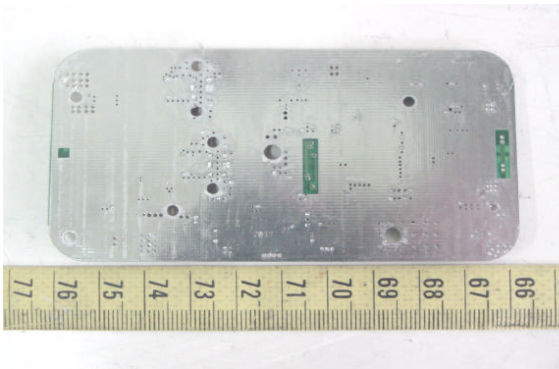
Solder View of Booster's PCB
