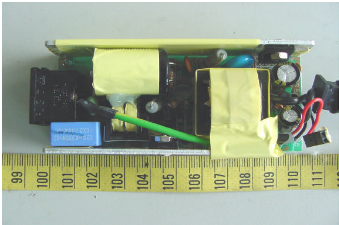
Component View of AC/DC Power Adaptor
