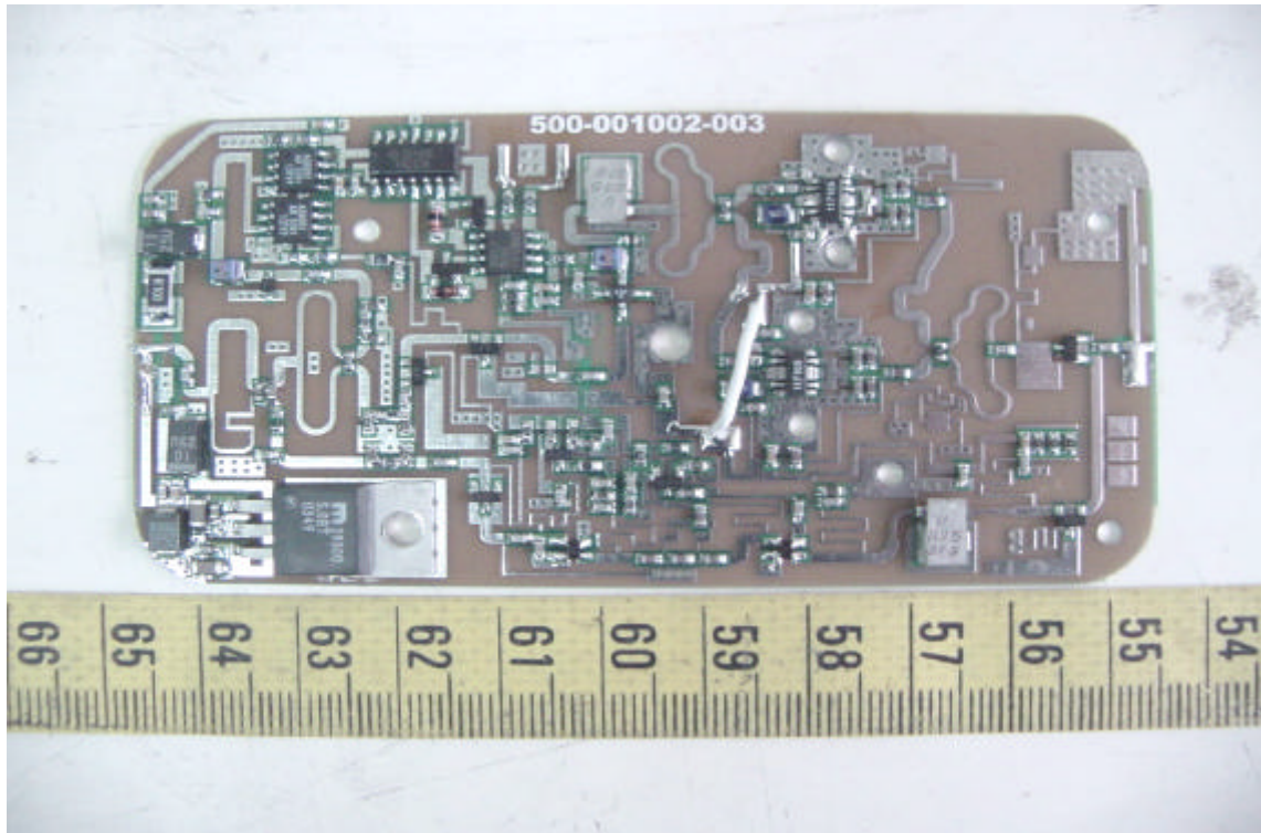
Component View of Booster's PCB
