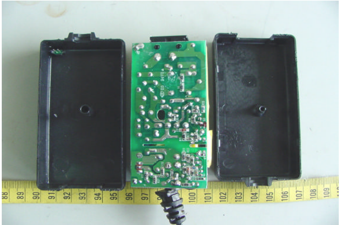
Internal View of AC/DC Power Adaptor
