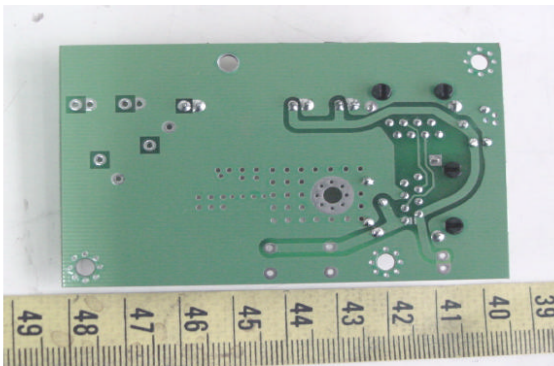
Solder View of DC to DC PCB
