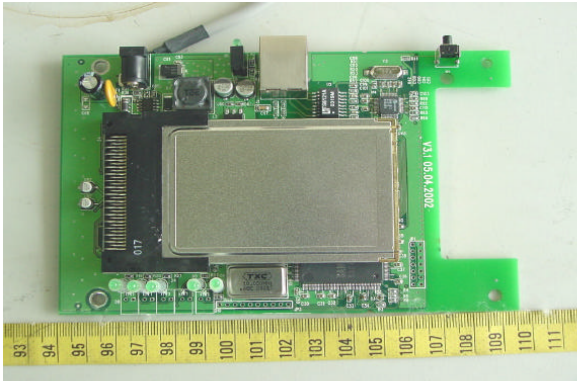
Internal View of Main PCB
