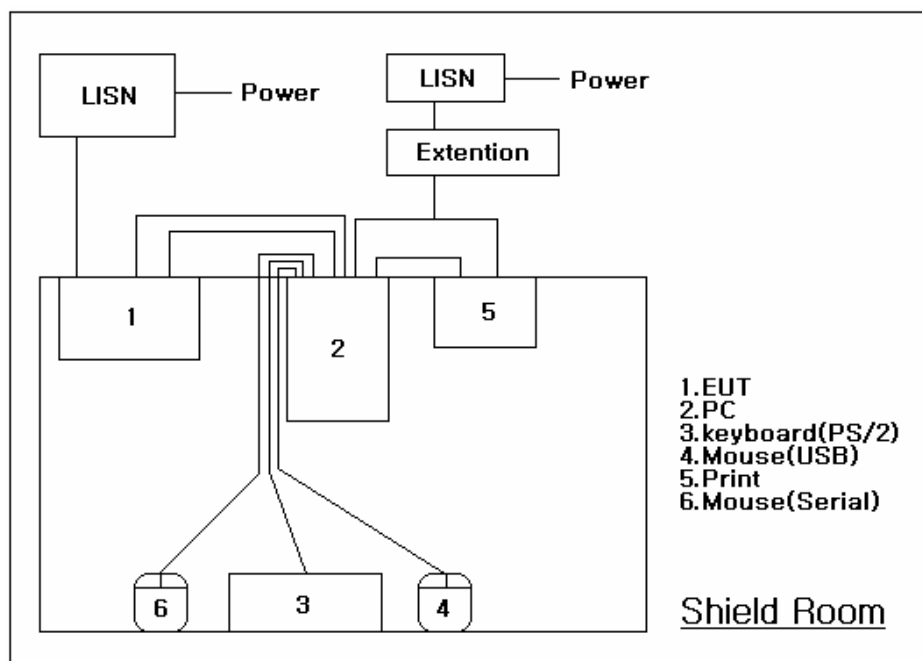
Conducted Emissions
