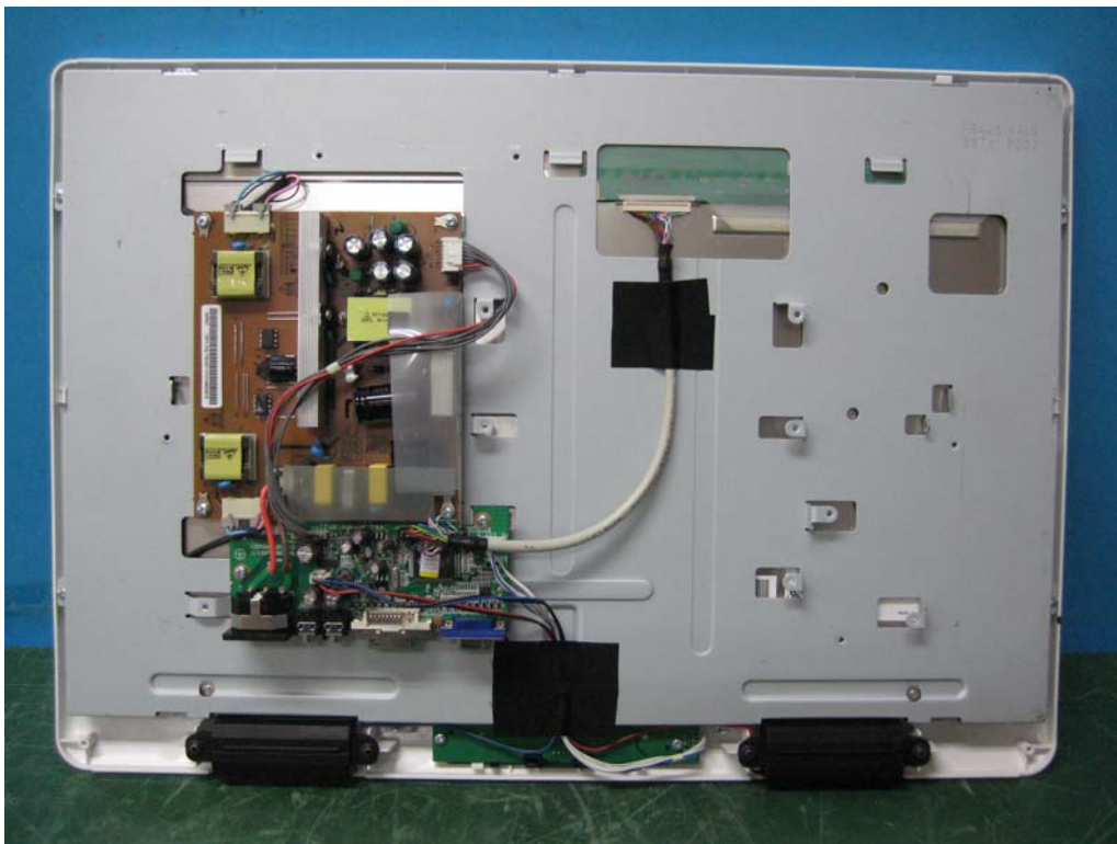
Inner View 2
