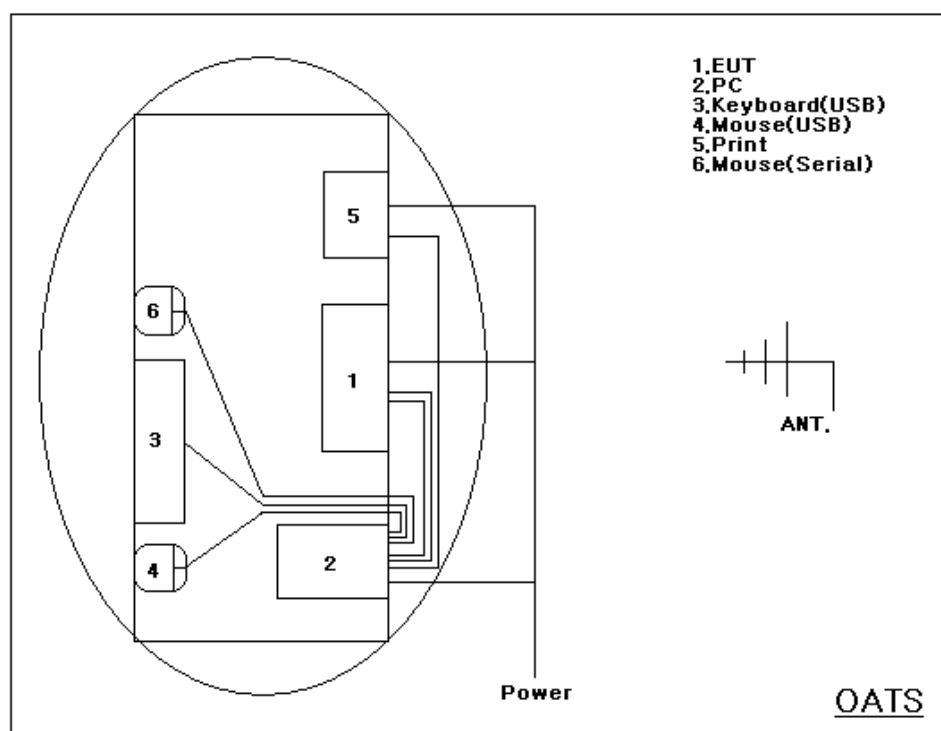
Radiated Emissions
