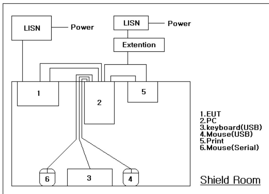
Conducted Emissions
