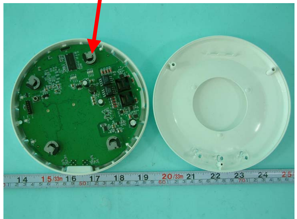
Internal PIFA Antenna (CAF94400) for 5GHz and 2.4GHz
