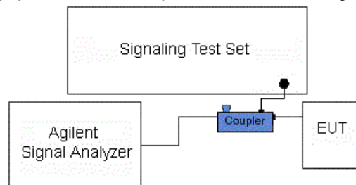
Figure 6-5. Test Instrument & Measurement Setup
