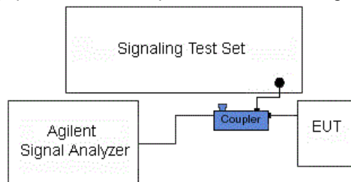
Figure 6-3. Test Instrument & Measurement Setup
