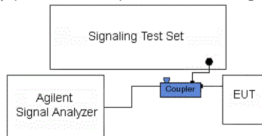
Figure 6-4. Test Instrument & Measurement Setup
