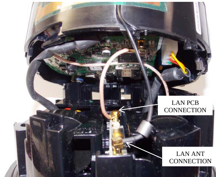
EA_Gatekeeper complete module with LAN RF filter connections
