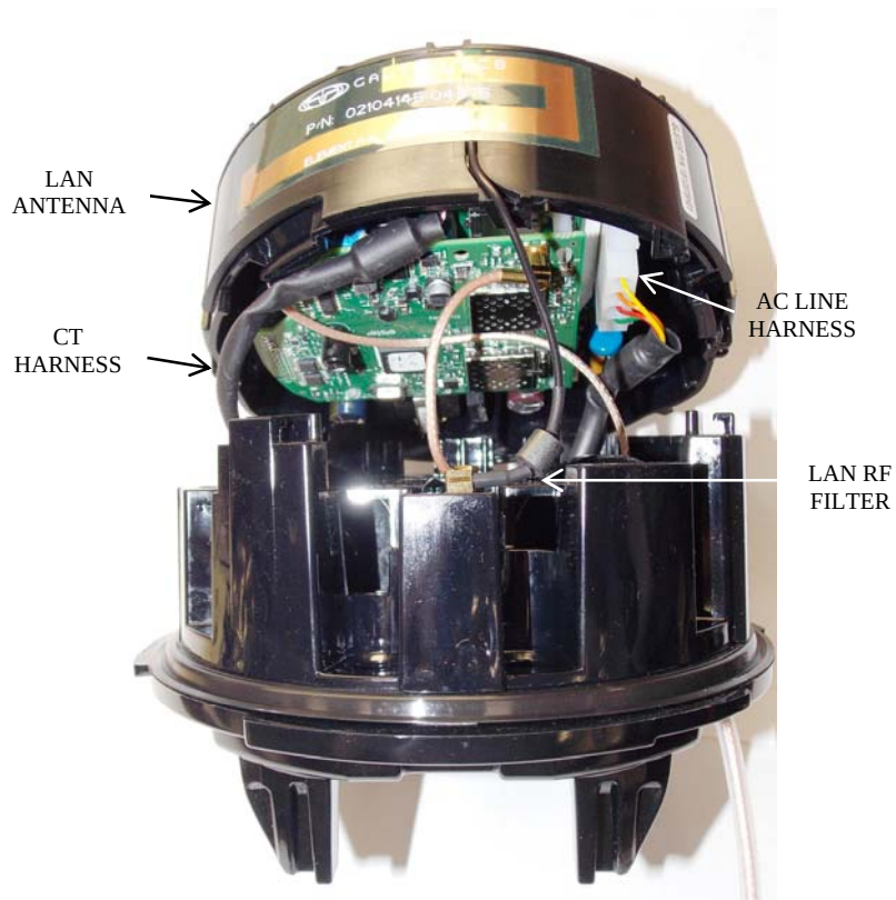
EA_Gatekeeper complete module with meter base
