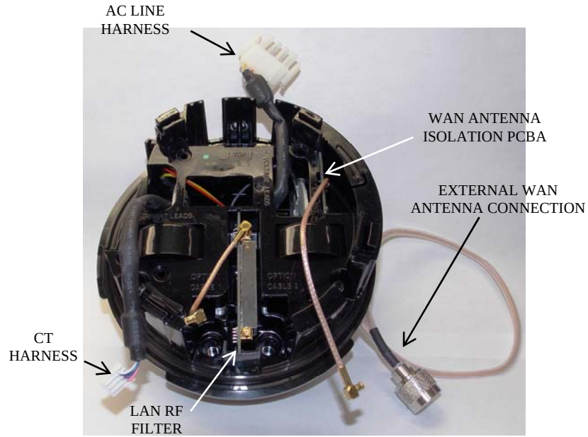
EA_Gatekeeper base (Form 2S)
