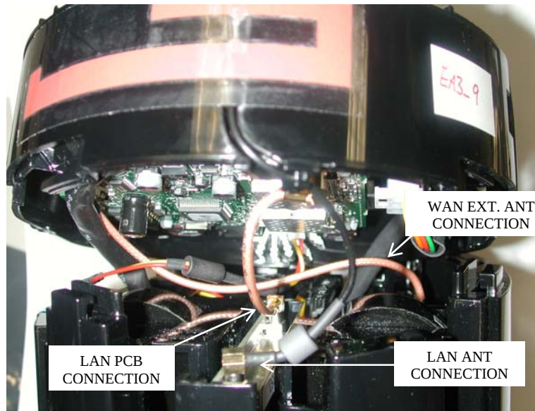
EA_Gatekeeper complete module with RF filter connections
