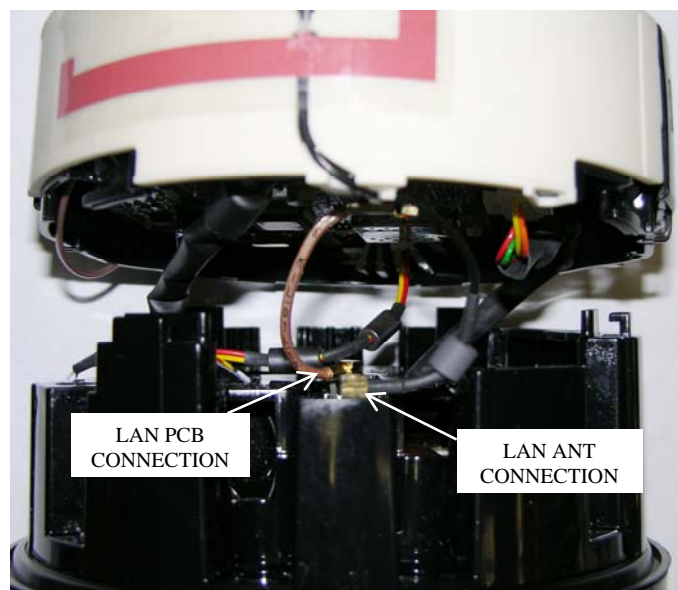
EA_Gatekeeper complete module with RF filter connections
