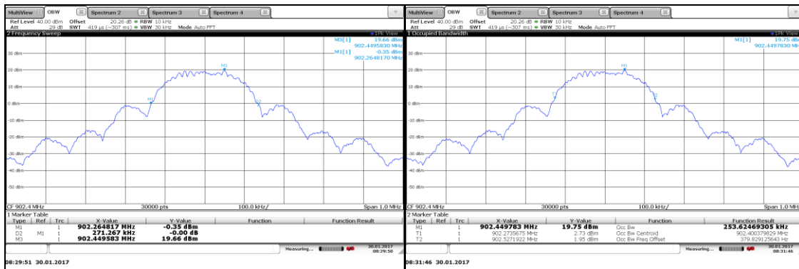
Figure 7.4.4.2-10: 99% OBW Low Channel – 200 kbps
