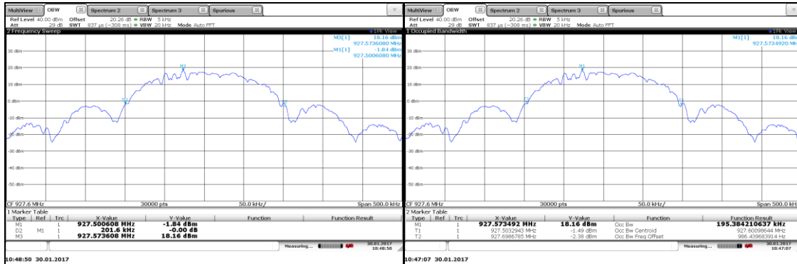
Figure 7.4.4.2-27: 20dB BW High Channel – 150 kbps
