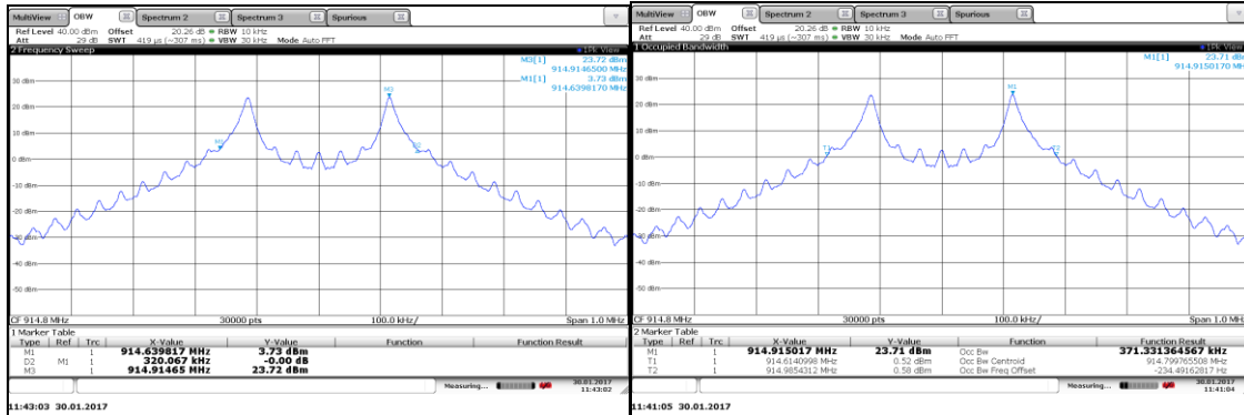
Figure 7.4.4.2-12: 99% OBW Mid Channel – 35.5 kbps
