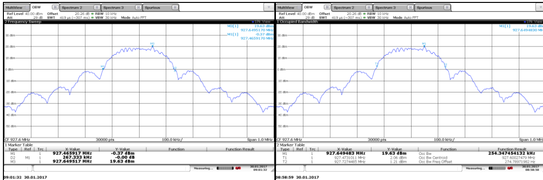
Figure 7.4.4.2-29: 20dB BW High Channel – 200 kbps
