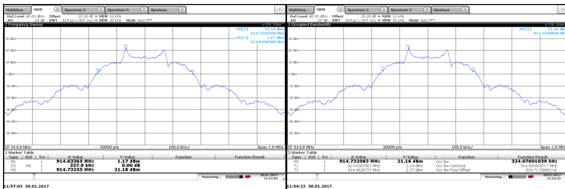
Figure 7.4.4.2-16: 99% OBW Mid Channel – 142.2 kbps
