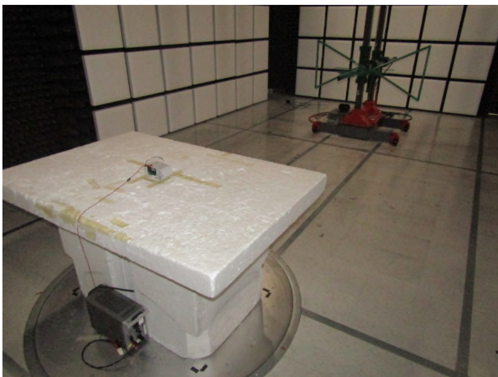
Figure 4: Radiated Emissions – Back – Below 1GHz – Form Factor 2
