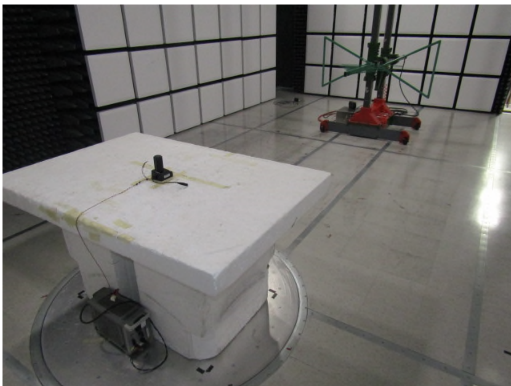
Figure 2: Radiated Emissions – Back – Below 1GHz – Form Factor 1
