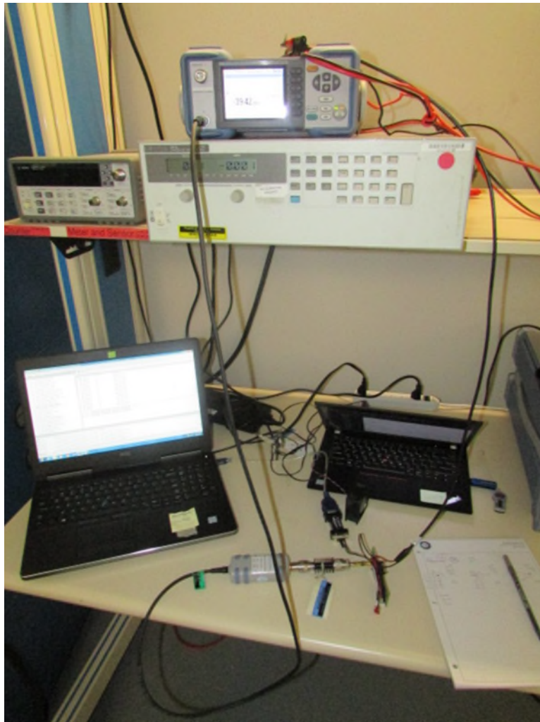
Figure 9: Conducted Emissions
