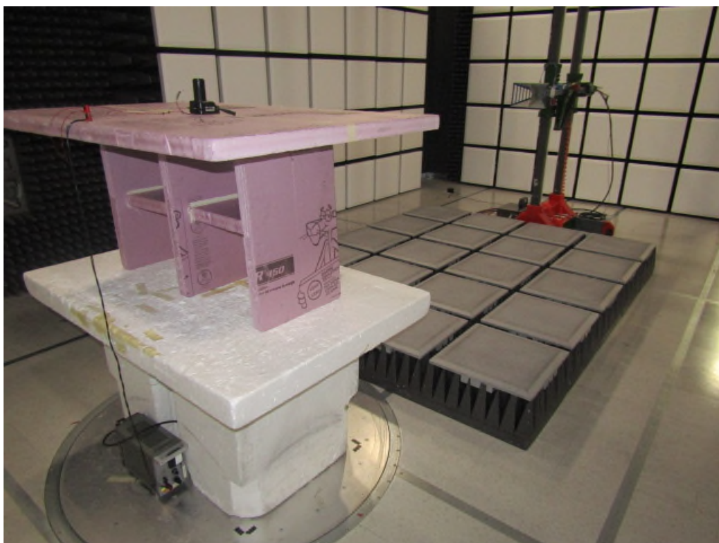
Figure 6: Radiated Emissions – Back – Above 1GHz – Form Factor 1
