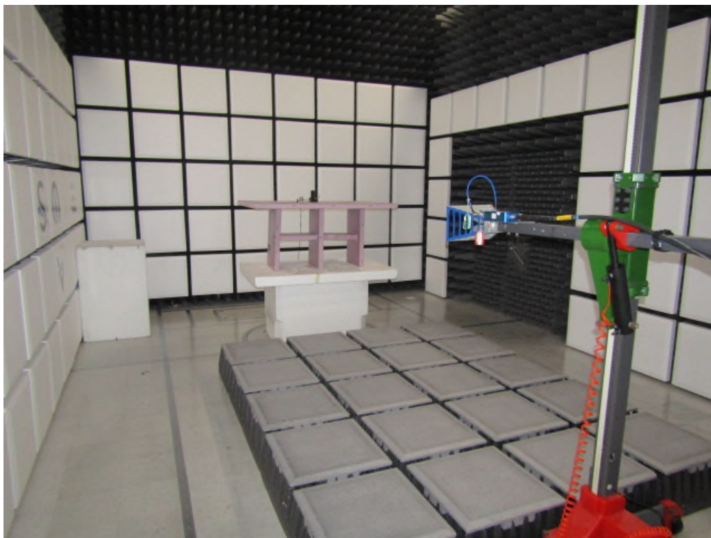
Figure 5: Radiated Emissions – Front – Above 1GHz – Form Factor 1
