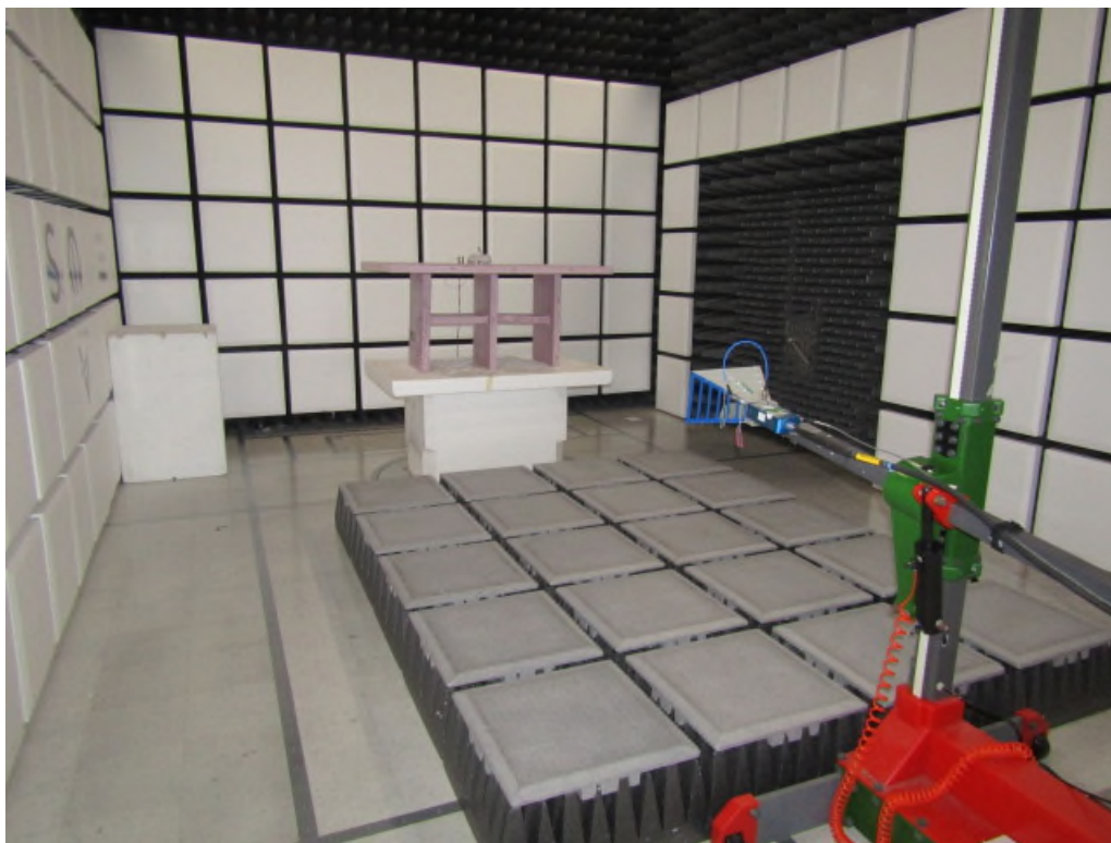
Figure 7: Radiated Emissions – Front – Above 1GHz – Form Factor 2
