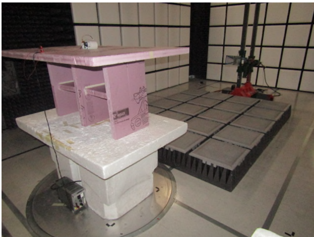
Figure 8: Radiated Emissions – Back – Above 1GHz – Form Factor 2
