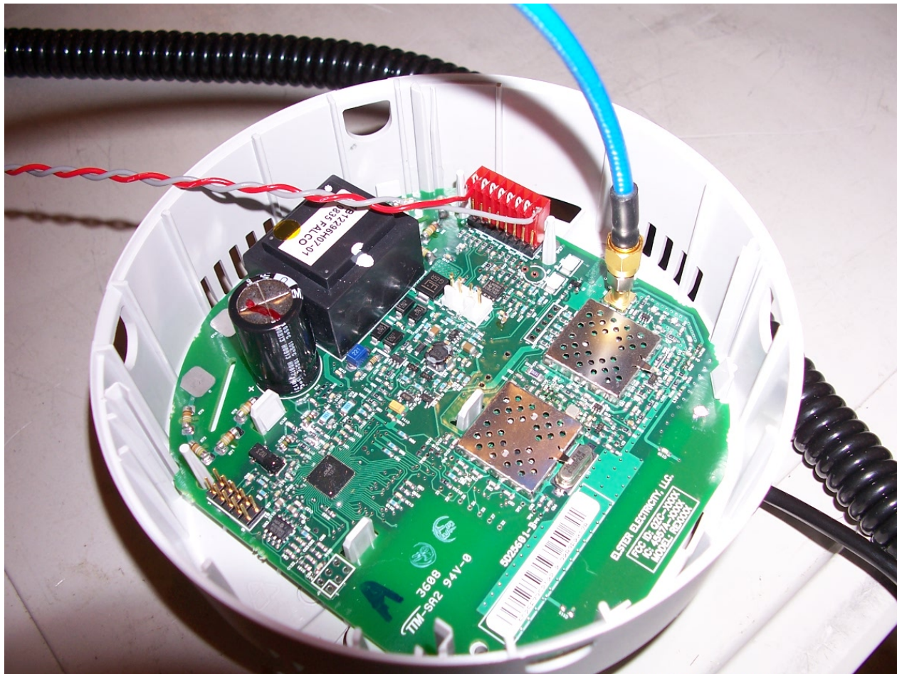
Close up view of EUT during RF Conducted Emissions Testing
