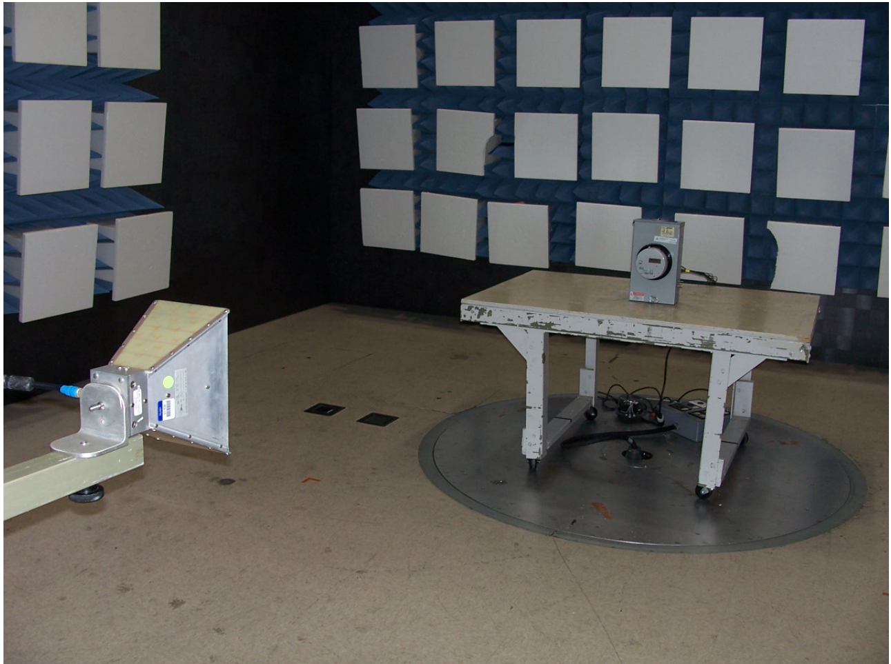
Radiated Emissions 1 - 10 GHz Test Setup
