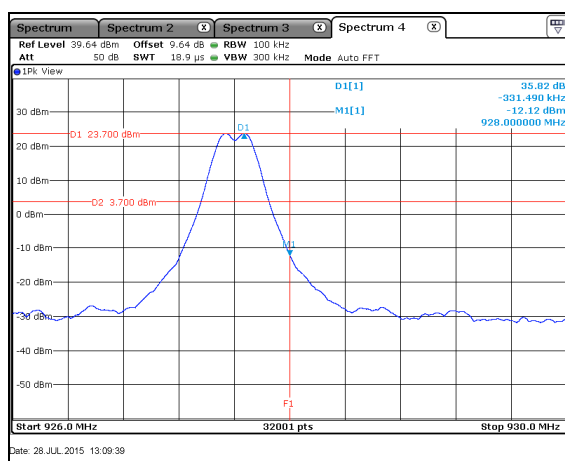
Figure 7.5.1.2-4: Upper Band-edge – 142.2kbps
