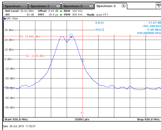
Figure 7.5.1.2-2: Upper Band-edge – 35.5kbps
