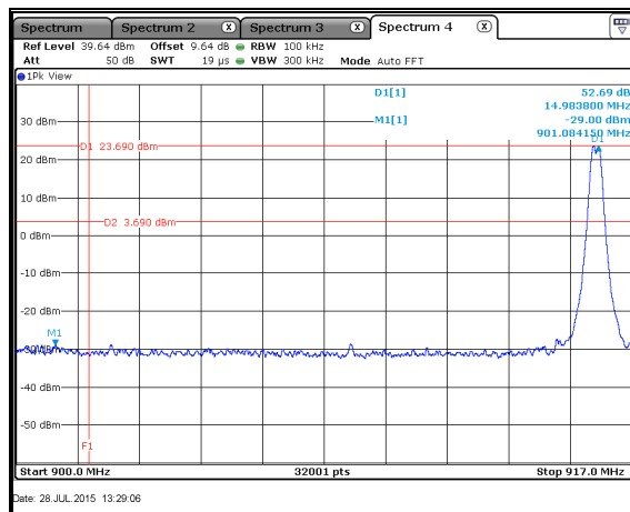
Figure 7.5.1.2-3: Lower Band-edge – 142.2kbps
