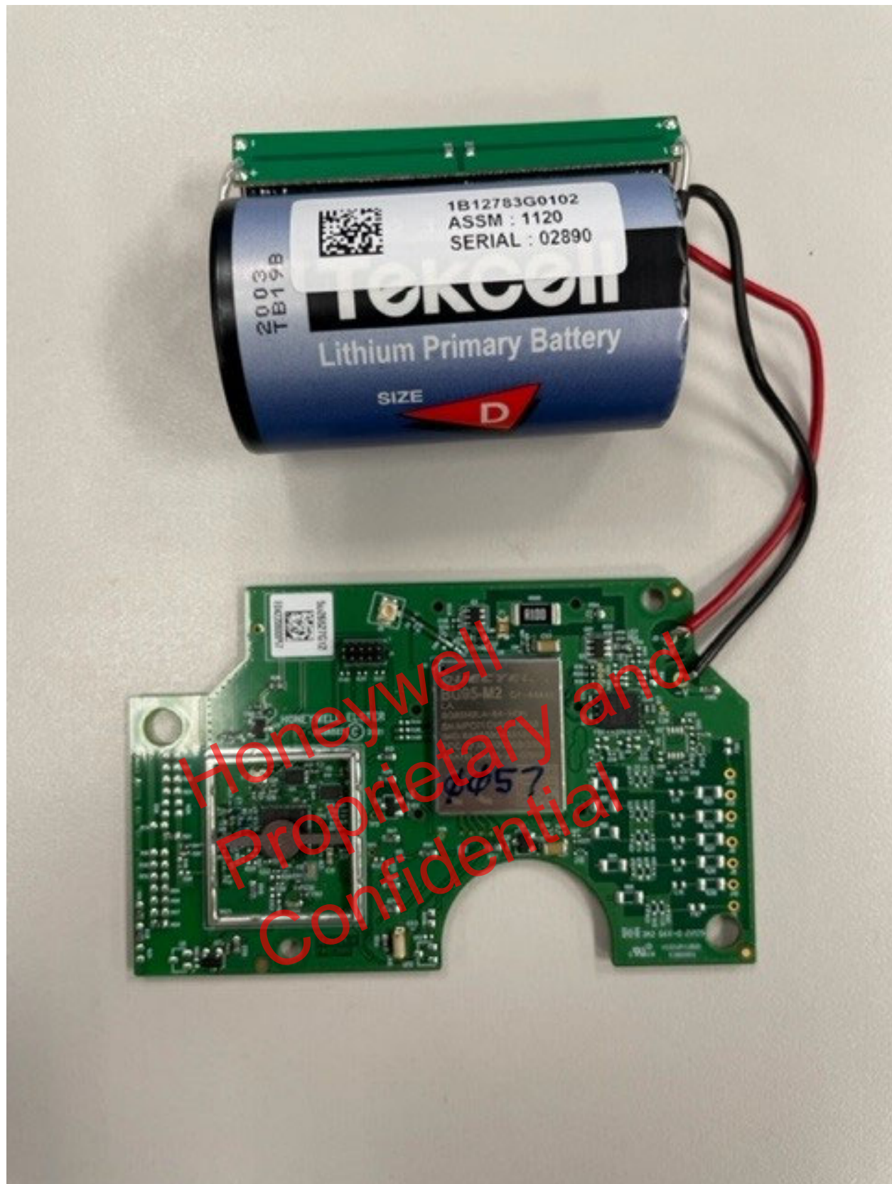
Integral Gas PCB top side with shield can lid removed
