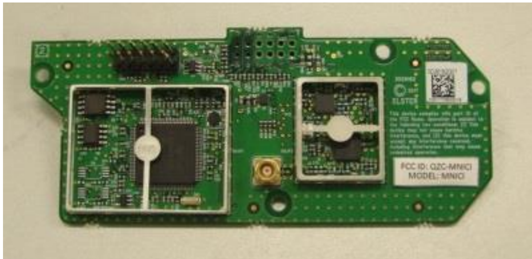
MNICI PCBA top view, shield can lids removed
