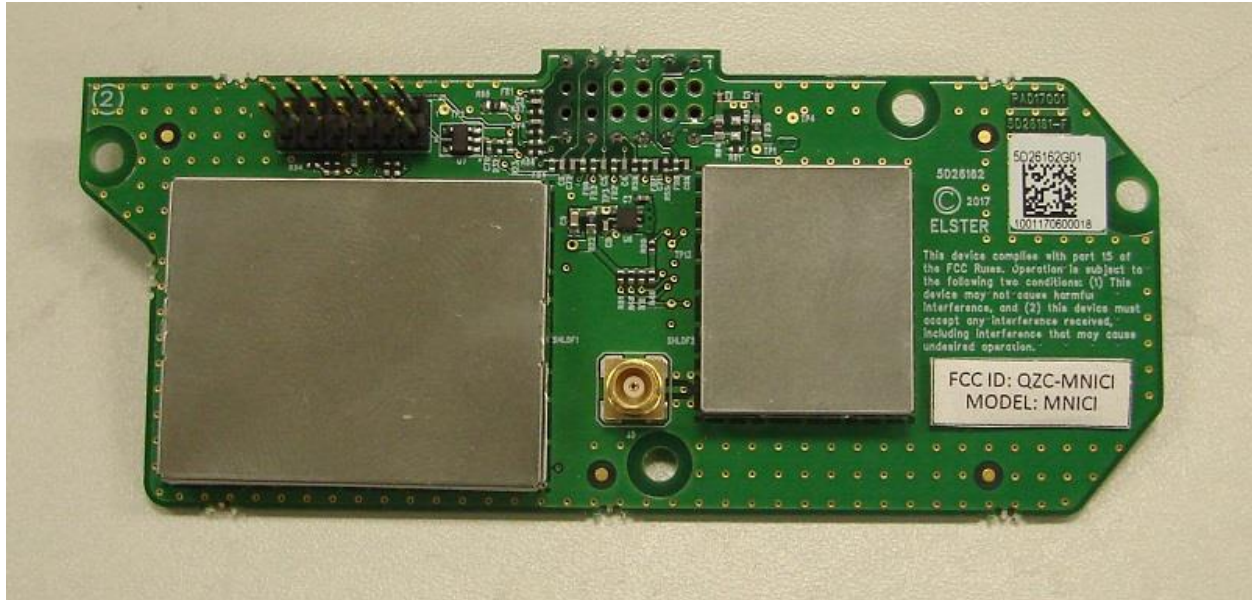
SynergyNet Mini Network Interface Card (MNICI) Printed Circuit Board Assembly (PCBA) top view
