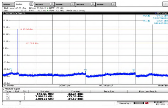
Figure 7.5.2.2-11: 30MHz-10GHz Mid Channel 150kbps
