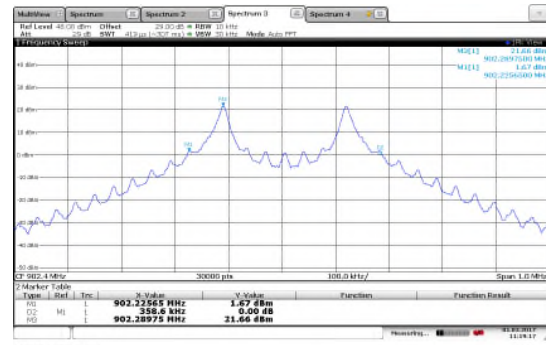
Figure 7.4.4.2-1: 20dB BW Low Channel 35.5kbps
