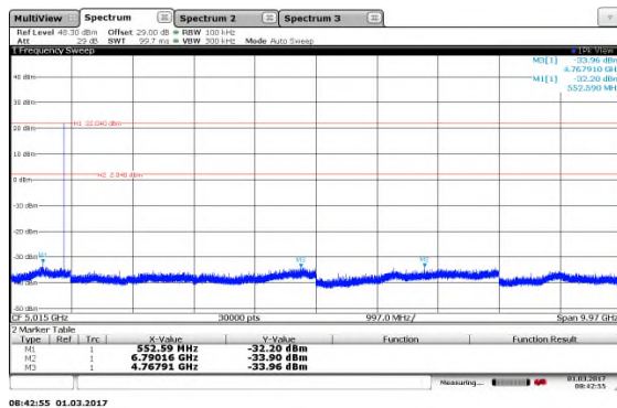
Figure 7.5.2.2-4: 30MHz–10GHz Low Channel 142.2kbps
