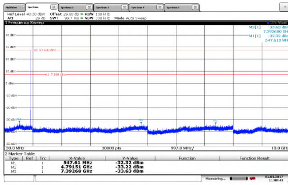
Figure 7.5.2.2-15: 30MHz–10GHz Mid Channel 200kpbs
