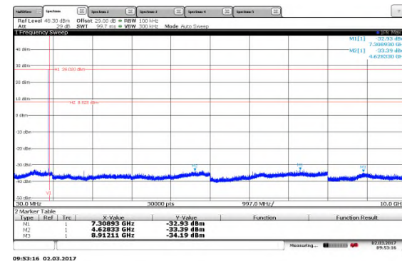
Figure 7.5.2.2-13: 30MHz-10GHz Low Channel 200kbps
