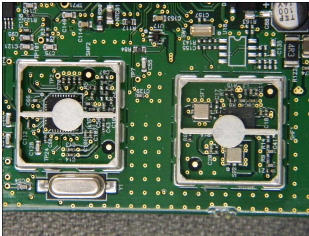
Figure 2: Internal Photo – Shields Removed
