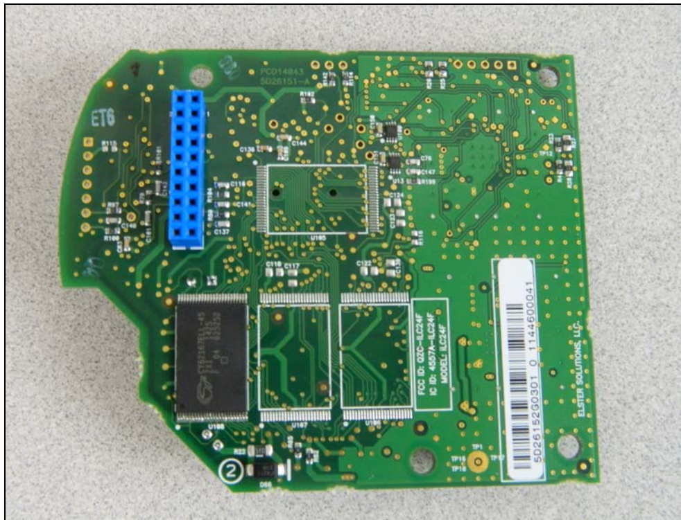
Figure 3: Internal Photo
