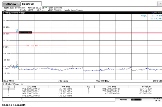
Figure 7.5.2.2-7: 30MHz-10GHz Low Channel 150kbps
