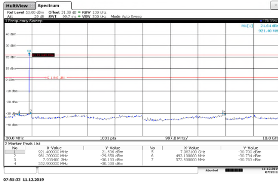
Figure 7.5.2.2-11: 30MHz-10GHz Mid Channel 200kbps
