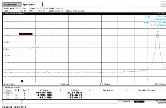
Figure 7.5.1.2-5: Lower Band-edge 150kbps
