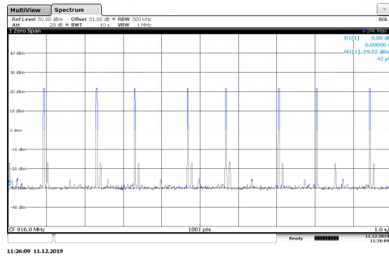
Figure 7.4.3.2-6: Number of Occurrences 150kbps
