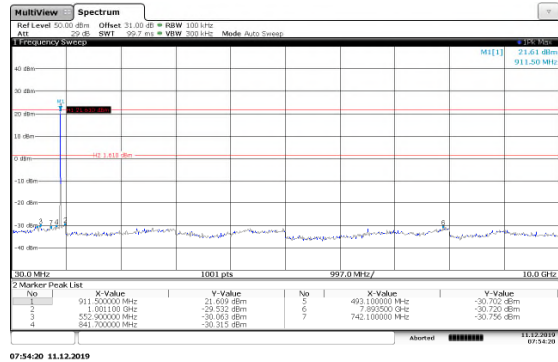
Figure 7.5.2.2-10: 30MHz-10GHz Low Channel 200kbps
