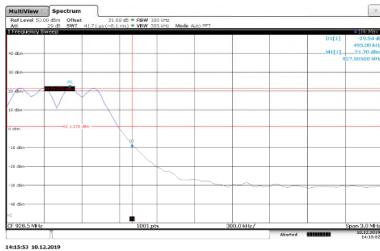
Figure 7.5.1.2-10: Upper Band-edge 35.5kbps
