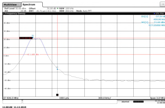
Figure 7.5.1.2-6: Upper Band-edge 150kbps
