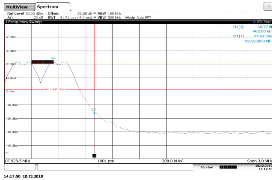
Figure 7.5.1.2-12: Upper Band-edge 142.2kbps
