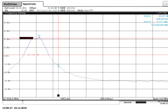
Figure 7.5.1.2-8: Upper Band-edge 200kbps
