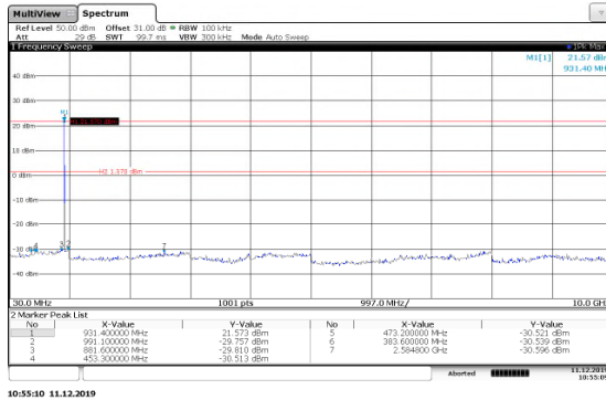
Figure 7.5.2.2-9: 30MHz-10GHz High Channel 150kbps
