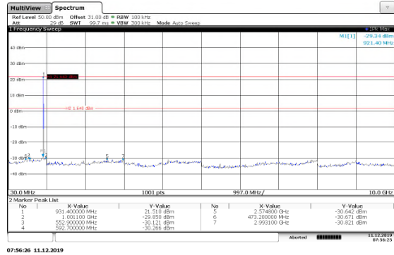
Figure 7.5.2.2-12: 30MHz-10GHz High Channel 200kbps
