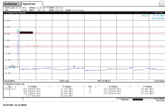
Figure 7.5.2.2-7: 30MHz-10GHz Low Channel 150kbps
