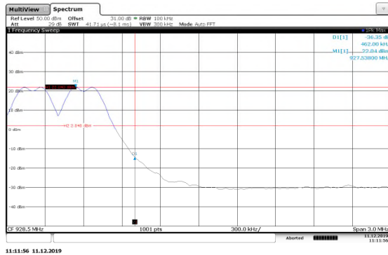
Figure 7.5.1.2-14: Upper Band-edge 150kbps
