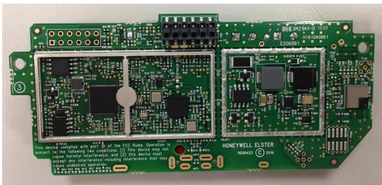
Figure 2: Top View without Shield – Model GNIC
