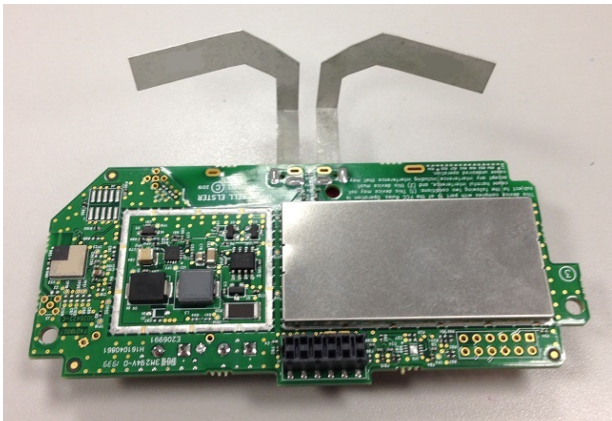
Figure 4: Antenna Installed
