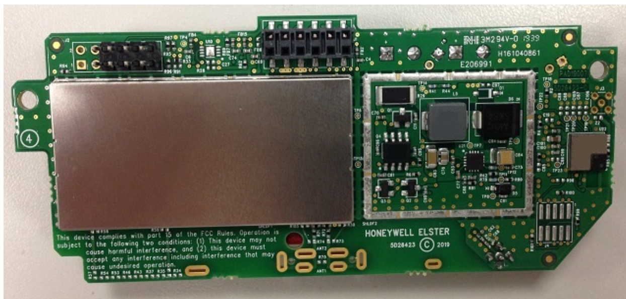
Figure 1: Top View with Shield
