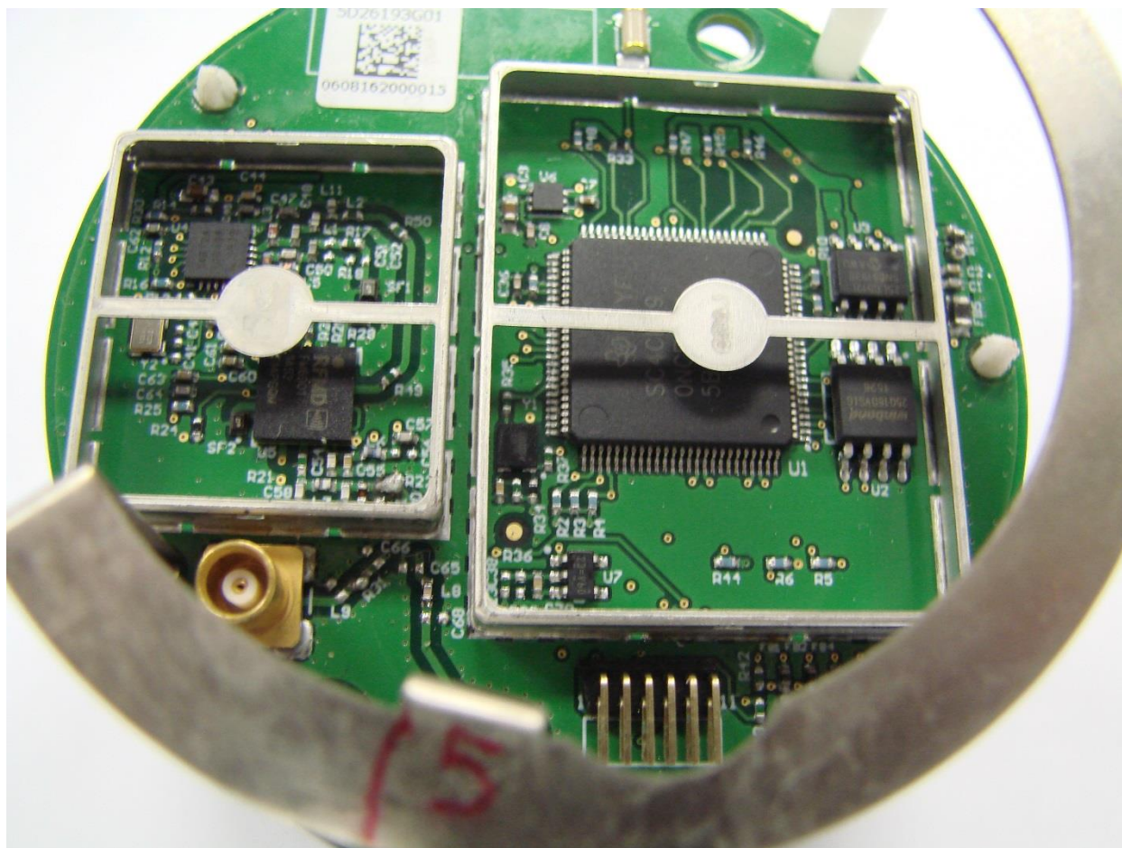
Radio PCBA, Top View, No Shields, Oblique 2
