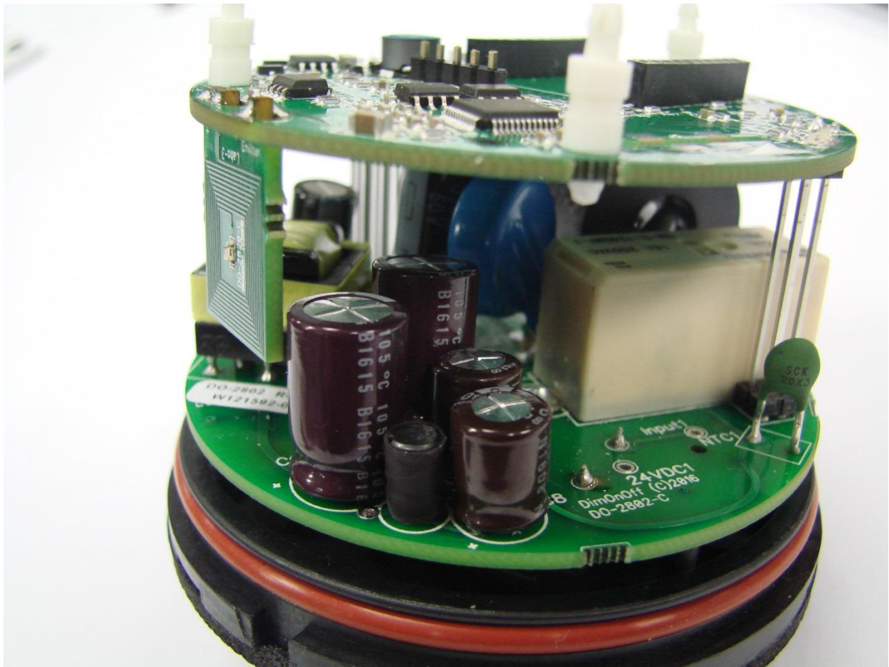
Lighting Module, Side View 1
