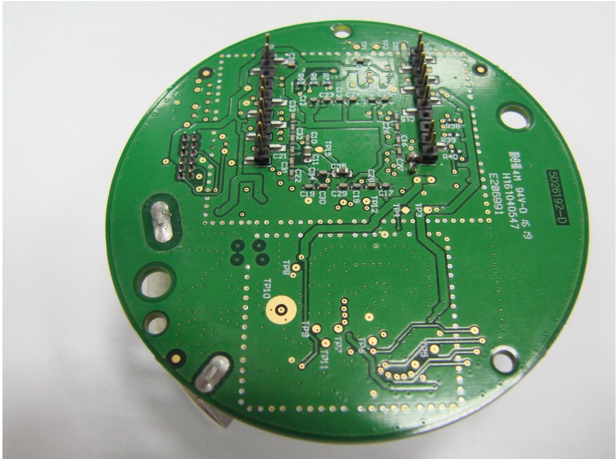
Radio PCBA, Bottom View
