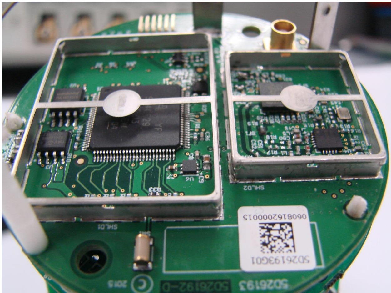
Radio PCBA, Top View, No Shields, Oblique 1
