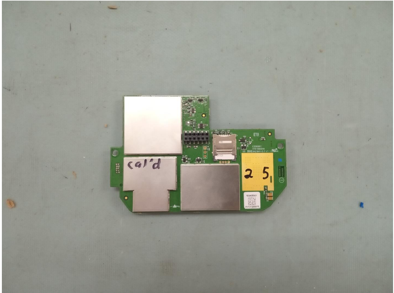
A4MGK4 PCBA Top Side, shield cans on
