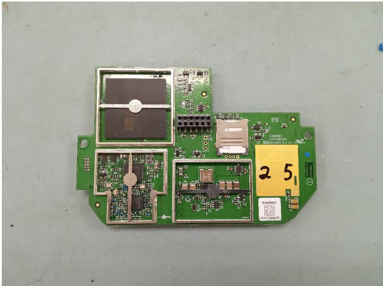
A4MGK4 PCBA Top Side, shield cans off
