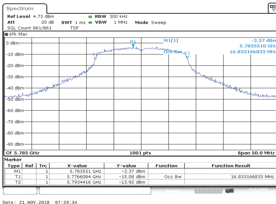
Plot 9: U-NII-3; middle channel
