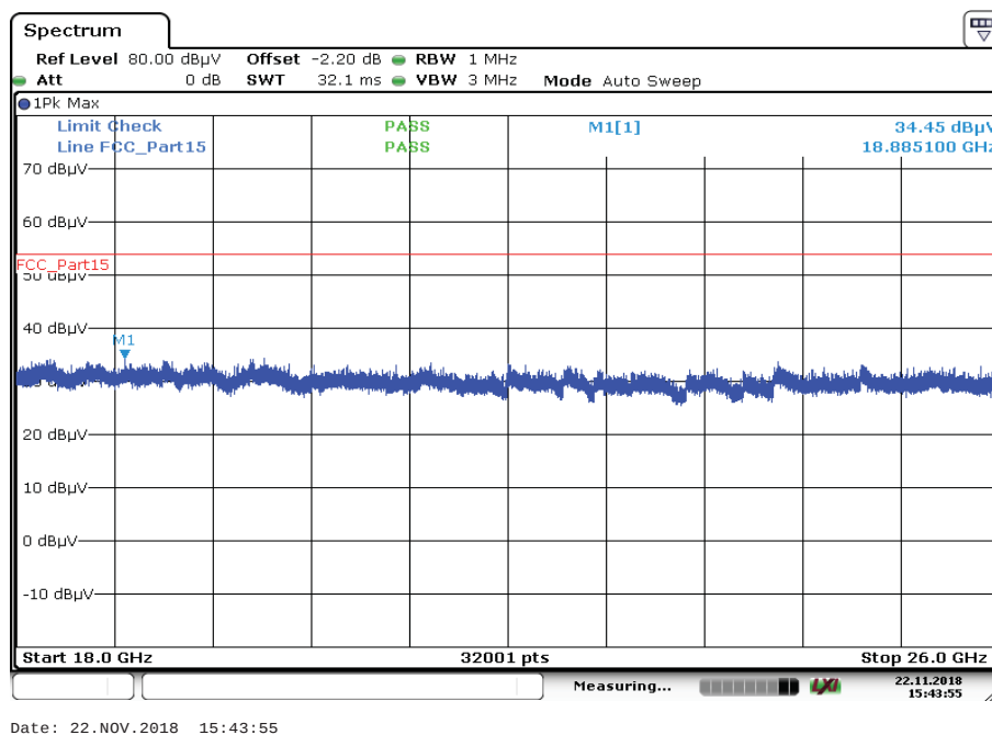
Plot 3: 18 GHz to 26 GHz, vertical & horizontal polarization
