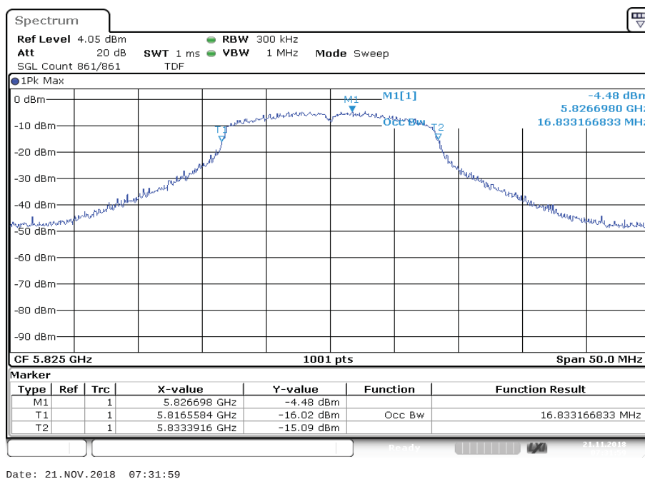
Plot 10: U-NII-3; highest channel
