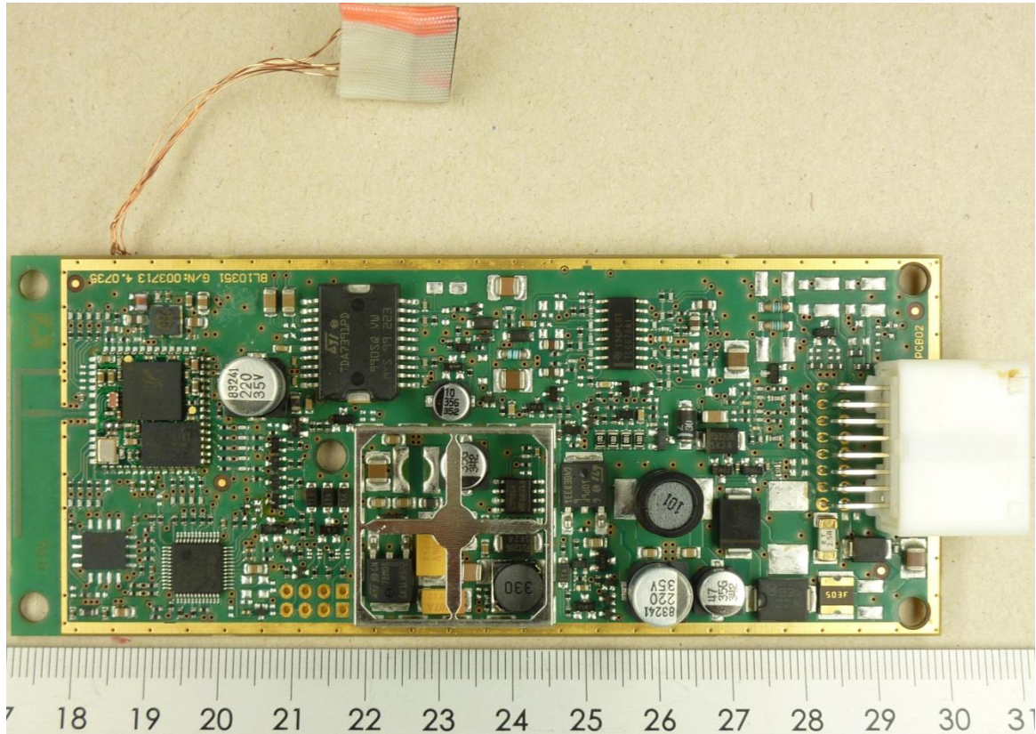
136031_8.jpg: EUT – Internal - Top View – No Shielding
