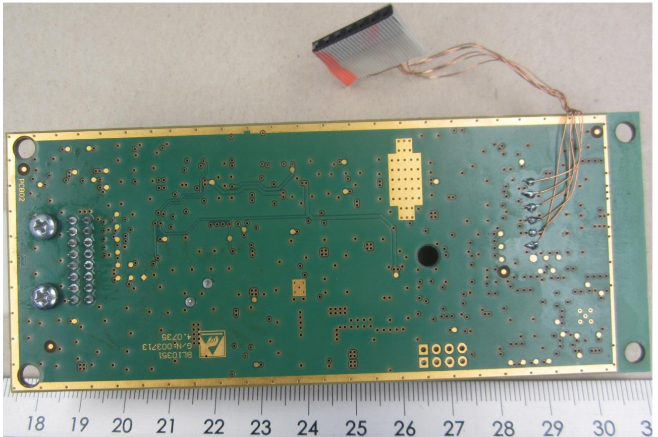
136031_7.jpg: EUT – Internal - Bottom View
