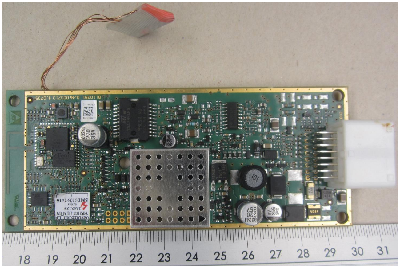
136031_4.jpg: EUT – Internal - Top View
