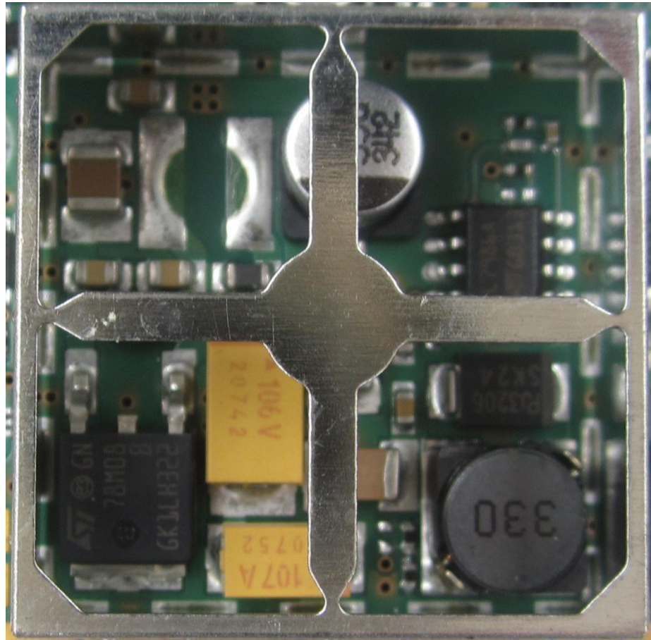
136031_6.jpg: EUT – Internal – Close-up shielded section
