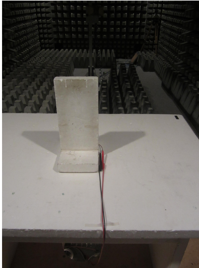
136031_17: Test setup - Radiated emission (fully anechoic chamber)
