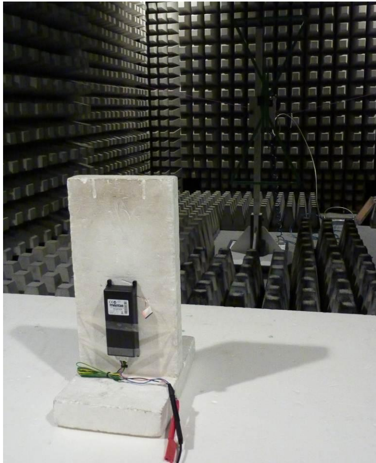
136031_16: Test setup - Radiated emission (fully anechoic chamber)
