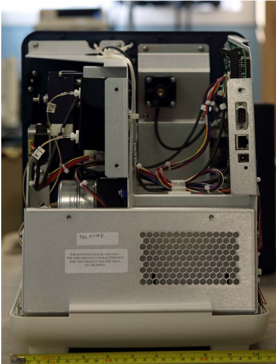
Rear
