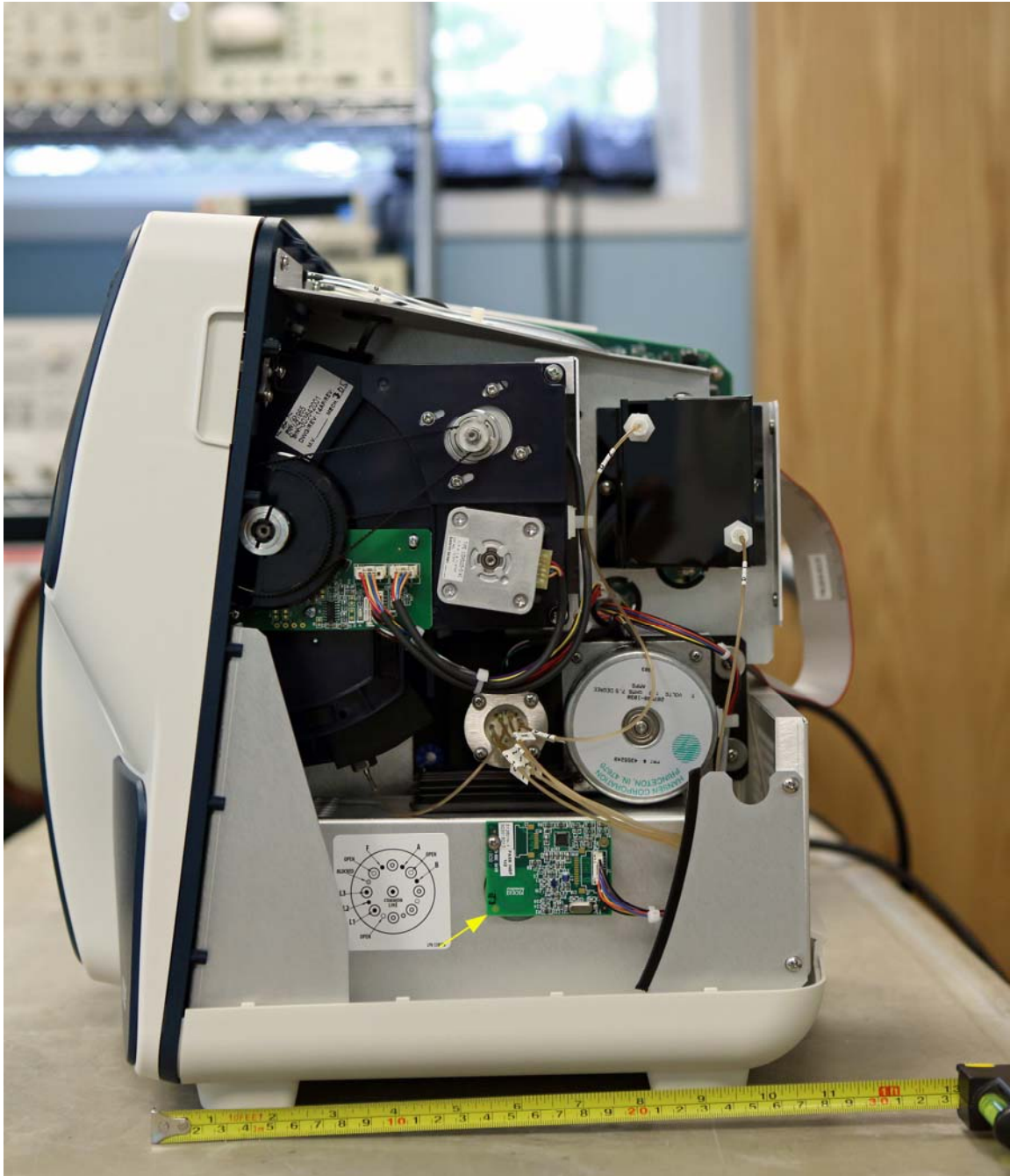
Right Side
