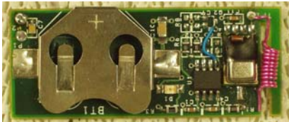
Front View of Transmitter Board
