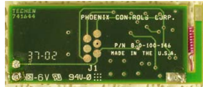
Back view of Transmitter Board
