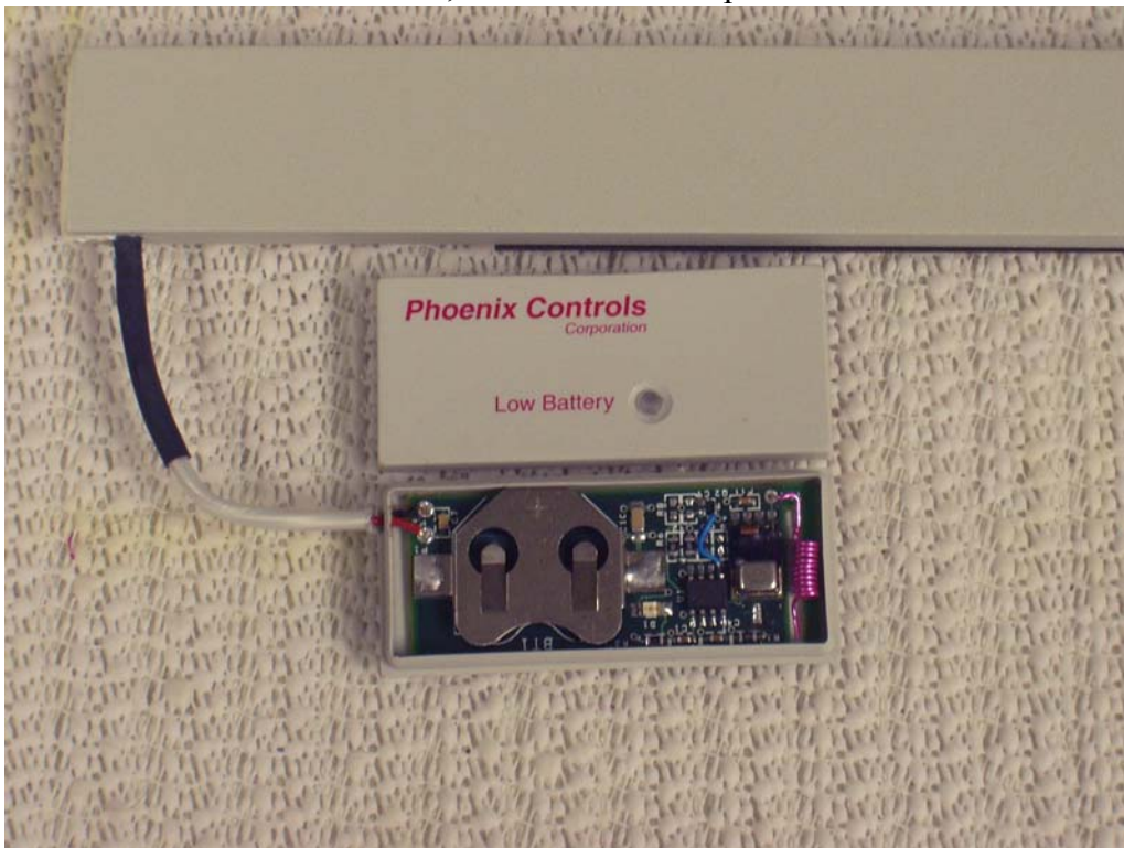
View of Board, as installed inside plastic case.
