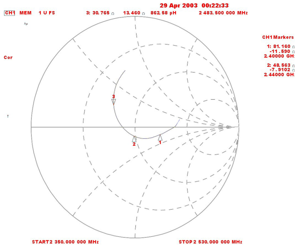
Fig 3. SMITH CHART
