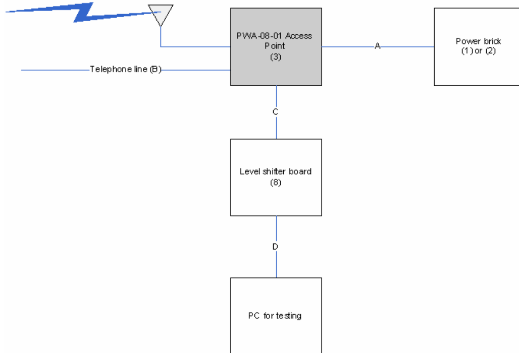
Figure 14 – Block diagram for testing EMC and modem on PWA-08-01
