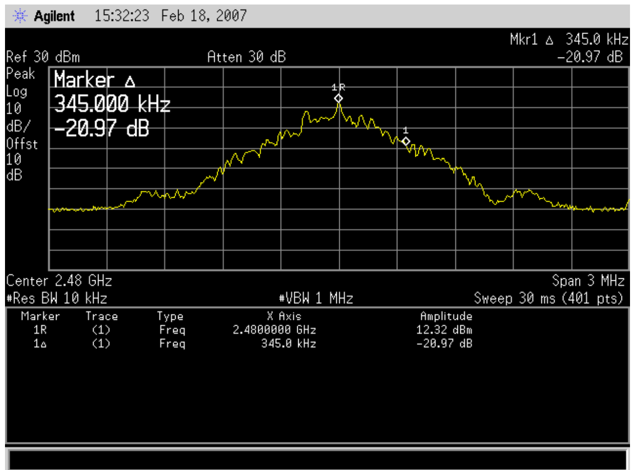
Figure 13 – 20dB down – high-band edge frequency (2480.000MHz + .345MHz = 2480.345 MHz).
