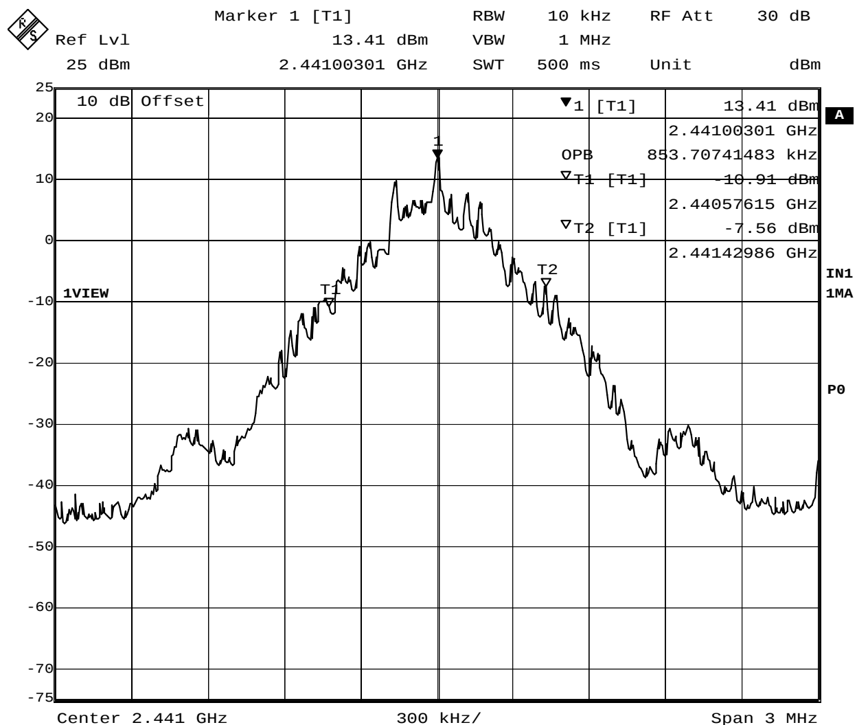
Figure 8 – Mid-band 99% Occupied Power Bandwidth
