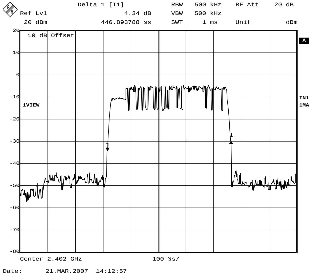
Figure 4 - Plot of EUT's Time on channel for one hop = 447 \mu s
