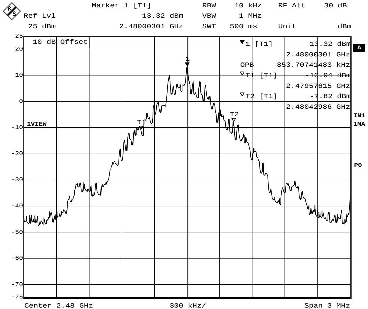
Figure 9 – High-band 99% Occupied Power Bandwidth
