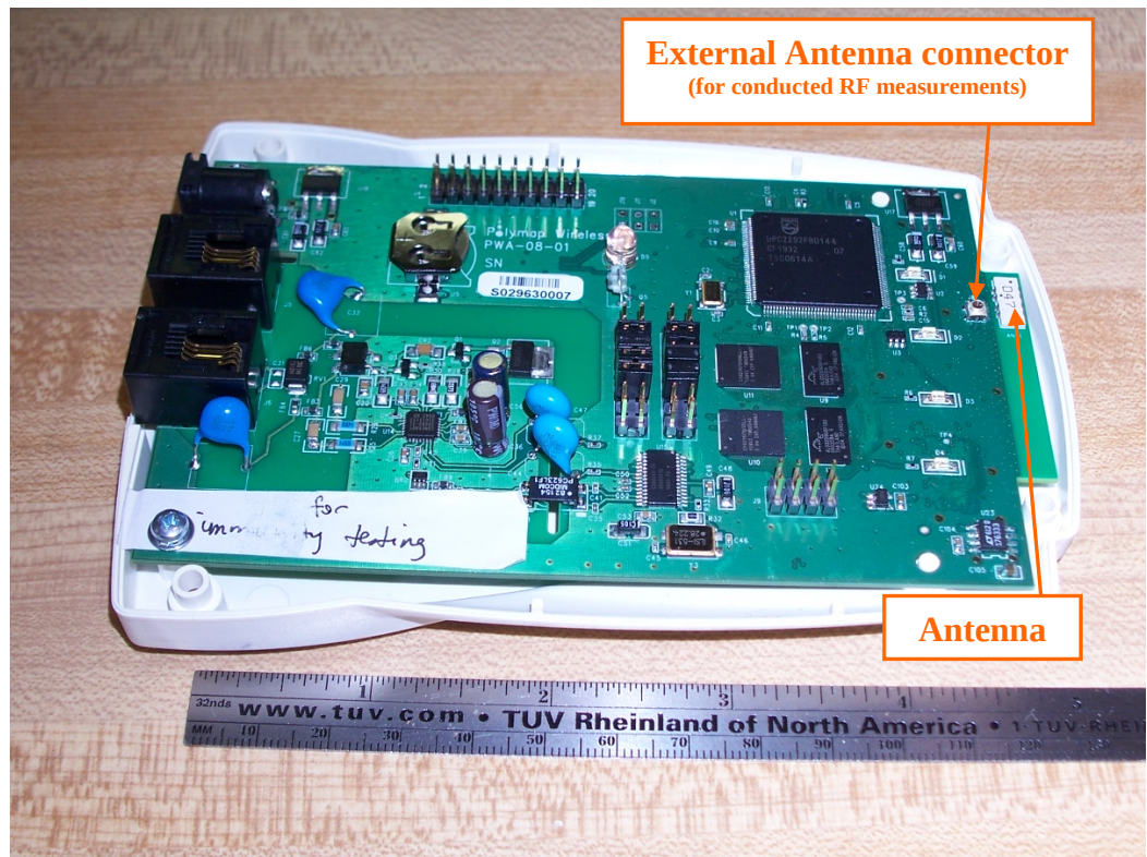
Figure 1 – Overall view of EUT
