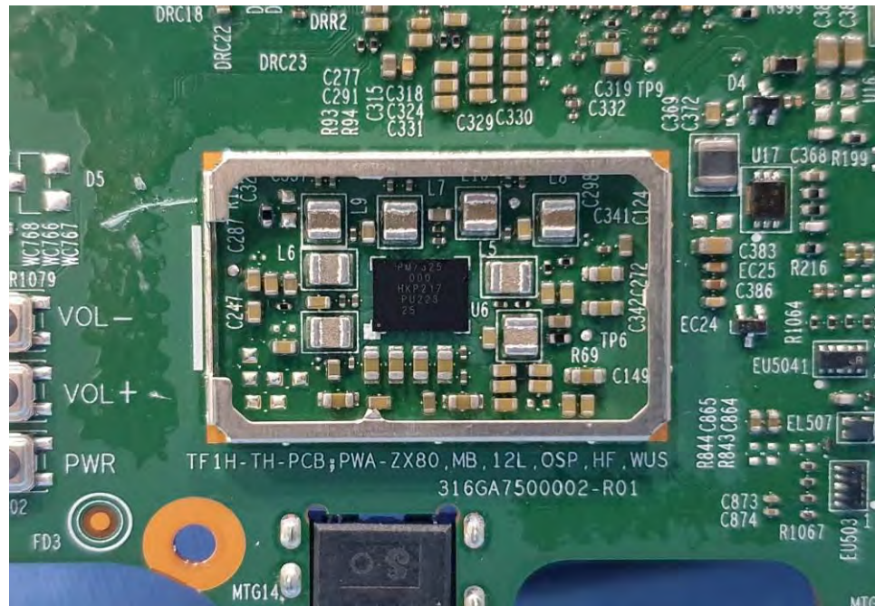
EUT Photo (45)
