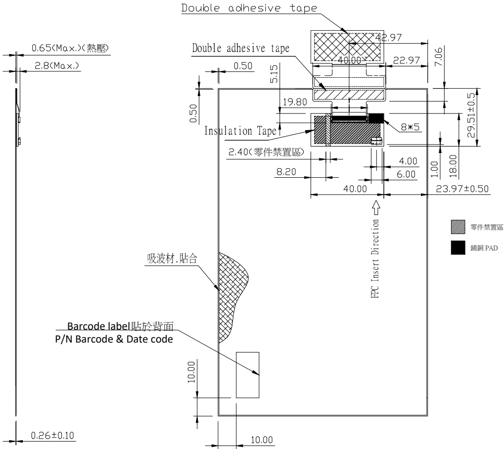
SIDE VIEW
