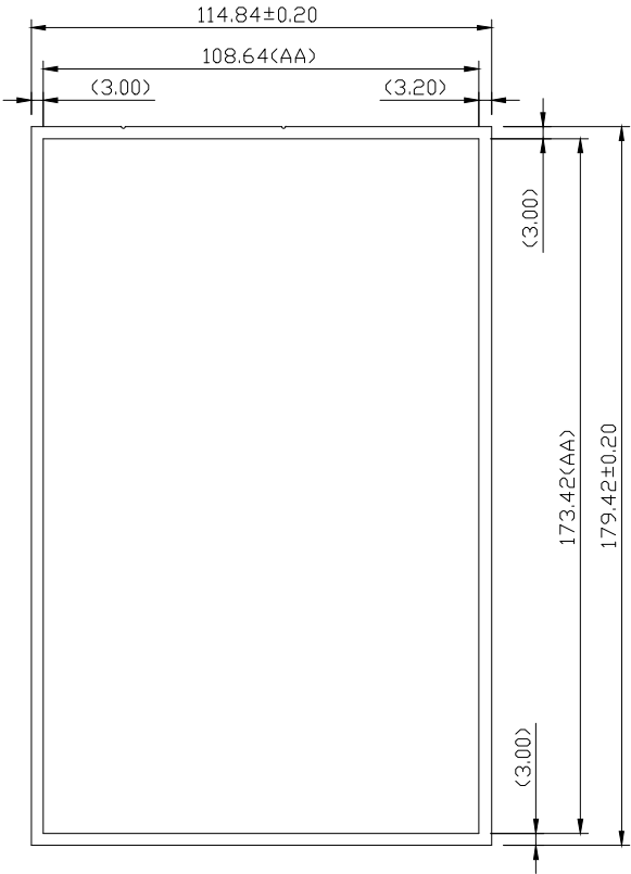
TOP VIEW
