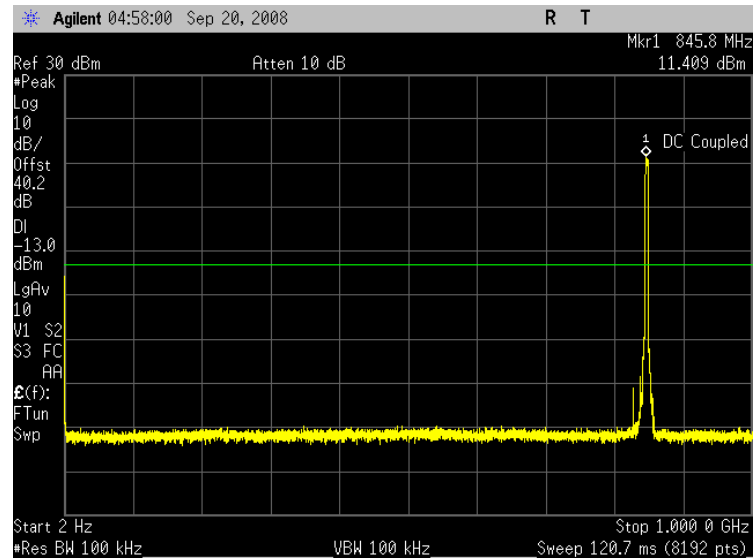
Plot 7.2 - 29(WCDMA, Rel99, Ch4233)
