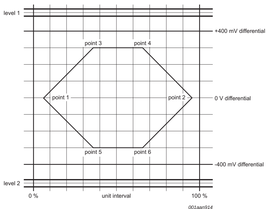
Fig 4. Transmit waveform at DP/DM
