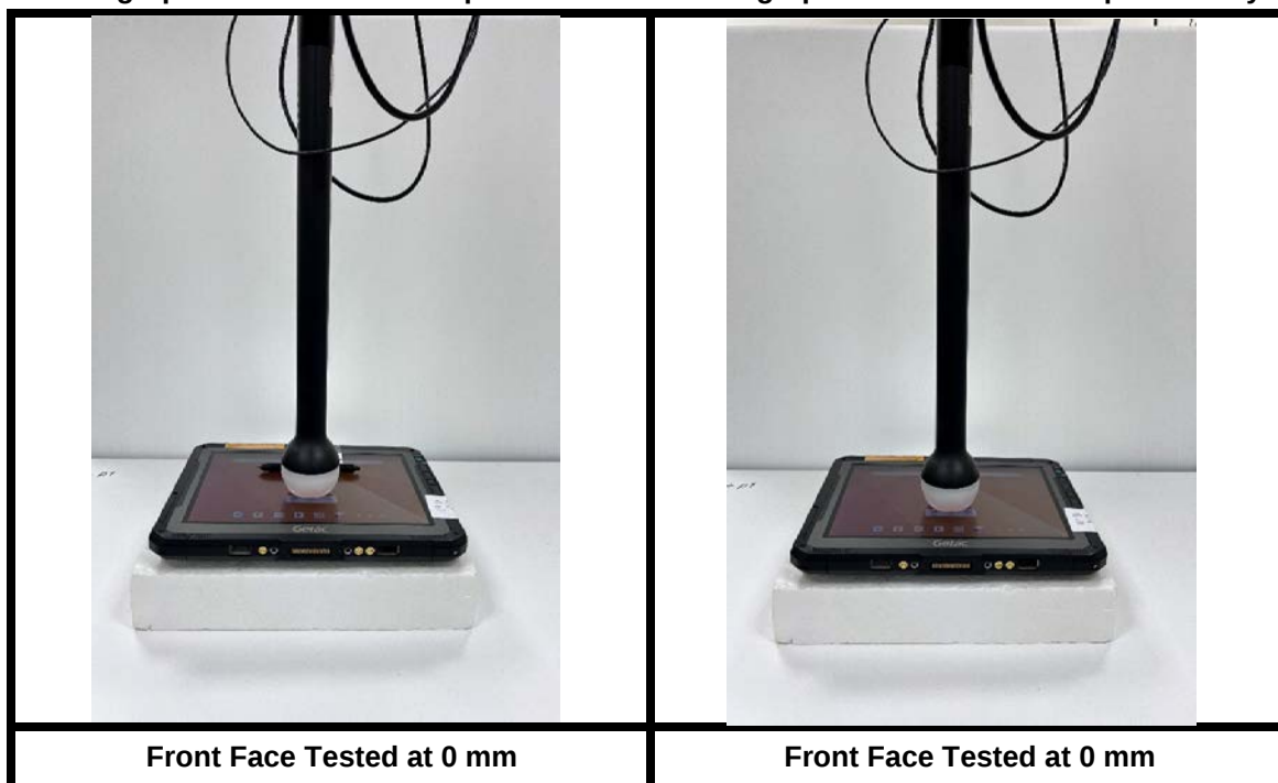
<Photographs of WPT Test Setup> 511KHz
